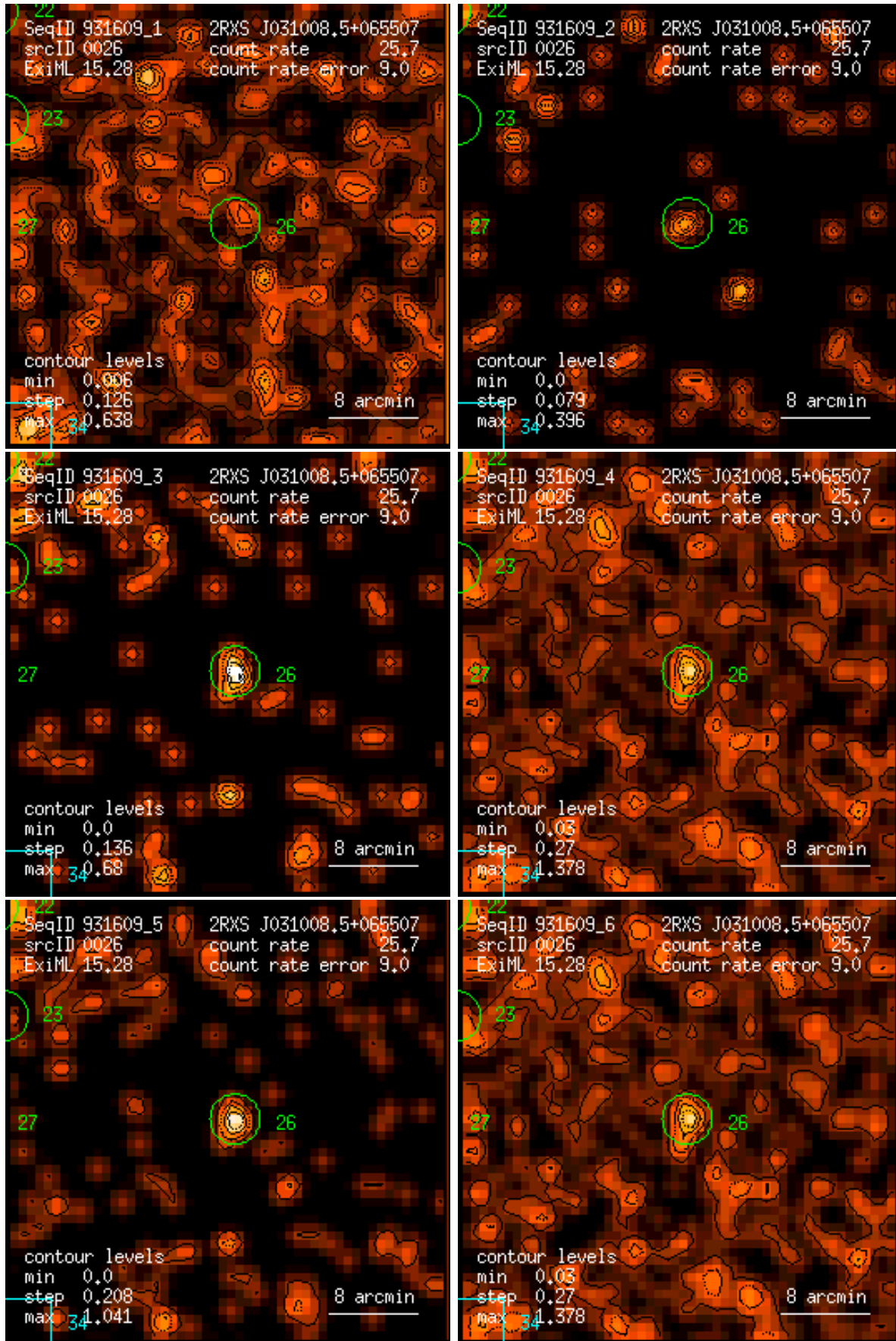
Figure 26: RASS 931609: detection 0026: band rate images, Gaussian filter: (1) PSPC channels 11 – 41, (2) 52 – 90, (3) 91 – 201, (4) 11 – 235, (5) 52 – 201, (6) 11 – 201. Broad band rates in counts/ks. Band rate contour levels in counts/ks/arcmin 2 .
