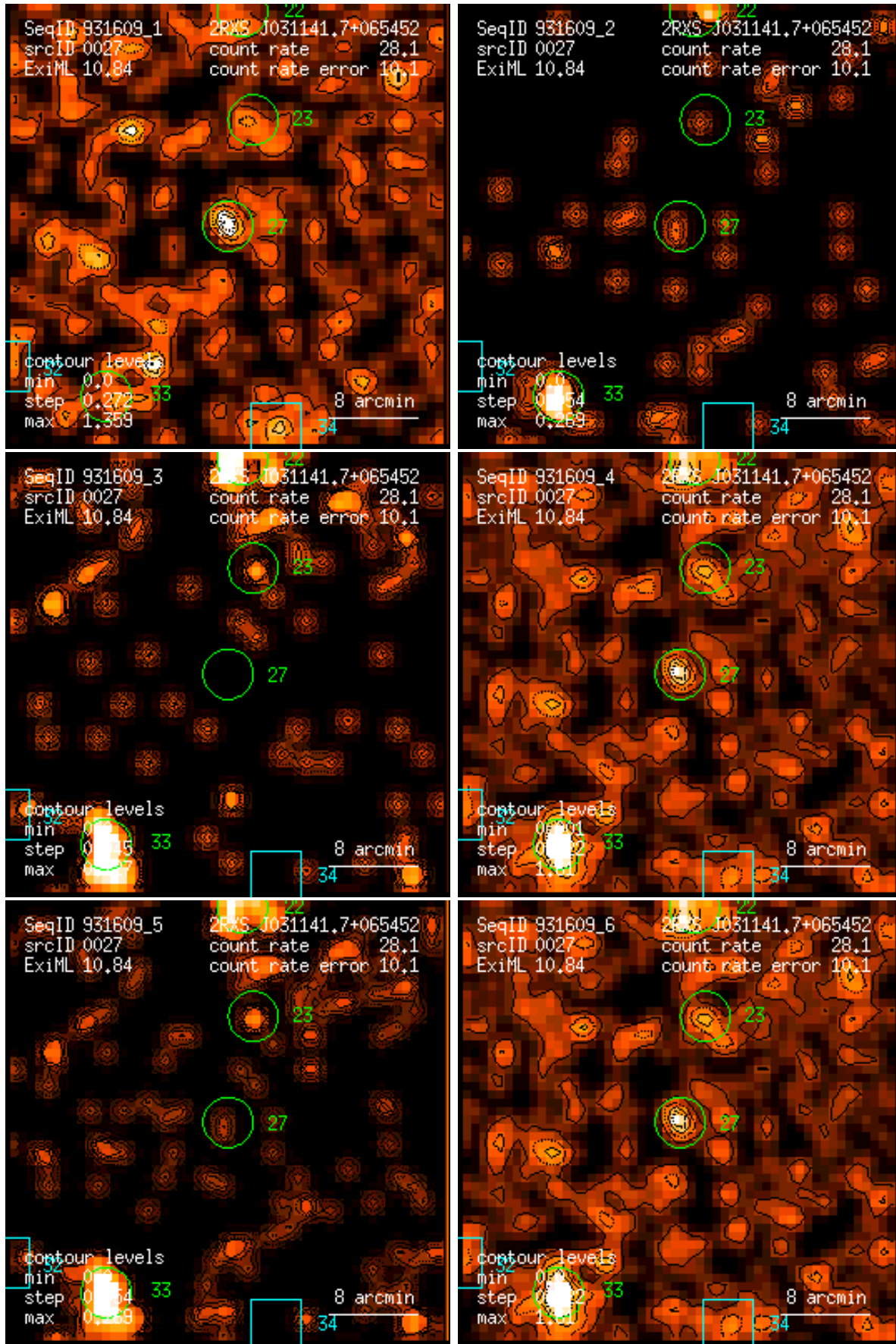
Figure 27: RASS 931609: detection 0027: band rate images, Gaussian filter: (1) PSPC channels 11 – 41, (2) 52 – 90, (3) 91 – 201, (4) 11 – 235, (5) 52 – 201, (6) 11 – 201. Broad band rates in counts/ks. Band rate contour levels in counts/ks/arcmin 2 .
