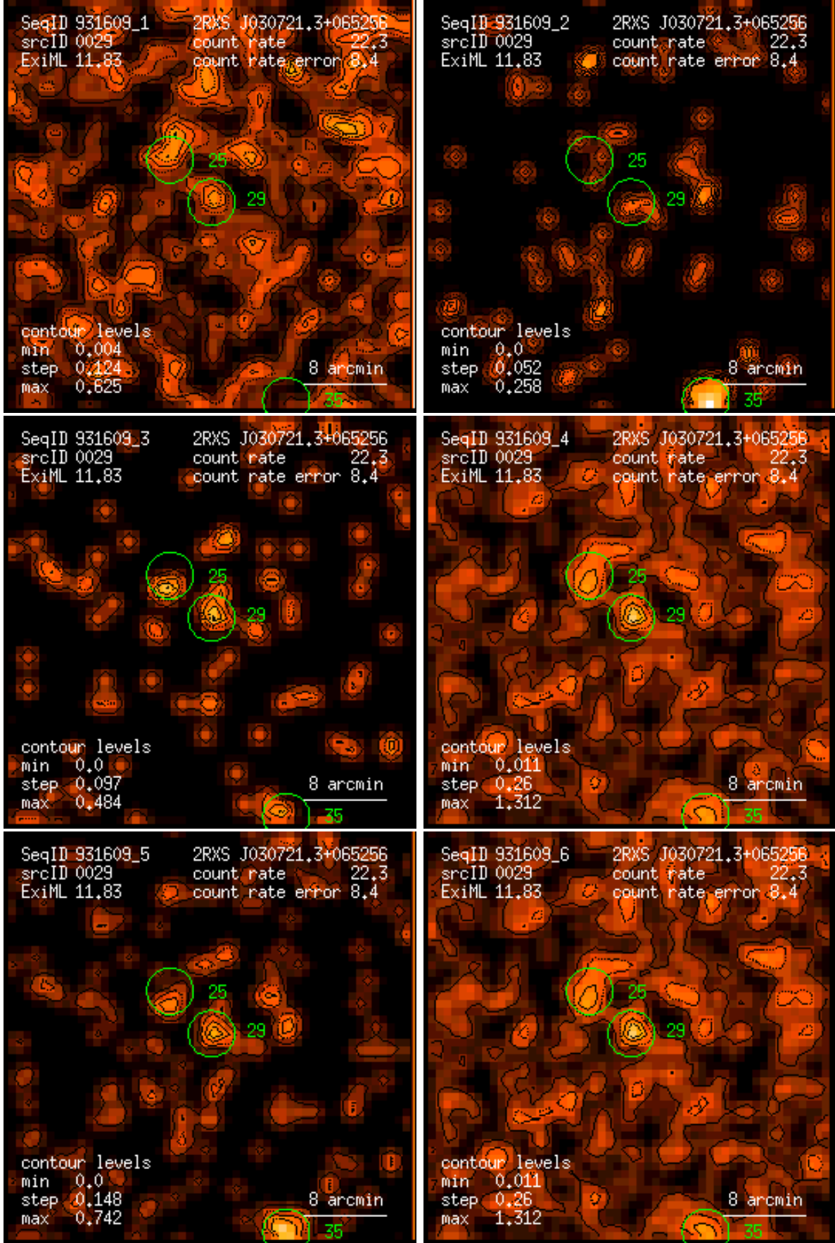
Figure 29: RASS 931609: detection 0029: band rate images, Gaussian filter: (1) PSPC channels 11 – 41, (2) 52 – 90, (3) 91 – 201, (4) 11 – 235, (5) 52 – 201, (6) 11 – 201. Broad band rates in counts/ks. Band rate contour levels in counts/ks/arcmin 2 .
