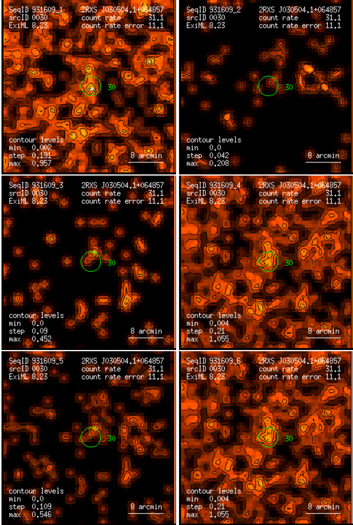
Figure 30: RASS 931609: detection 0030: band rate images, Gaussian filter: (1) PSPC channels 11 – 41, (2) 52 – 90, (3) 91 – 201, (4) 11 – 235, (5) 52 – 201, (6) 11 – 201. Broad band rates in counts/ks. Band rate contour levels in counts/ks/arcmin 2 .
