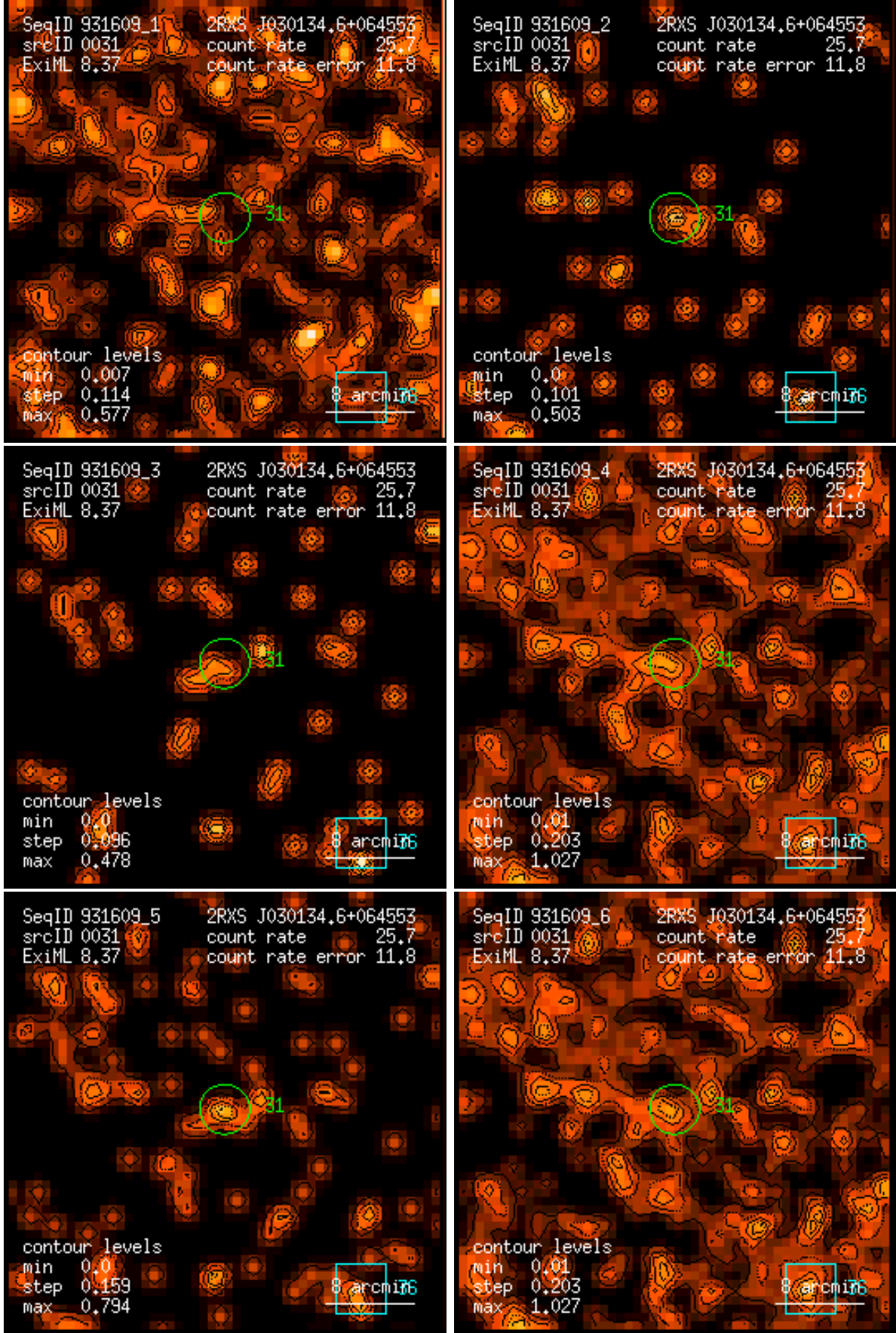
Figure 31: RASS 931609: detection 0031: band rate images, Gaussian filter: (1) PSPC channels 11 – 41, (2) 52 – 90, (3) 91 – 201, (4) 11 – 235, (5) 52 – 201, (6) 11 – 201. Broad band rates in counts/ks. Band rate contour levels in counts/ks/arcmin 2 .
