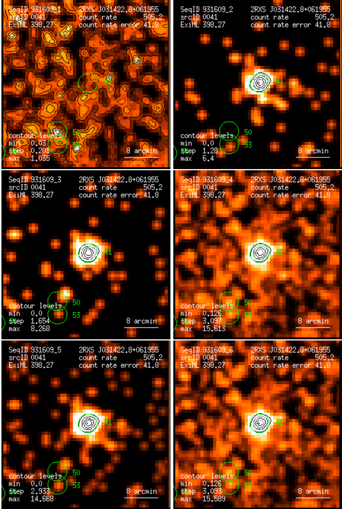
Figure 41: RASS 931609: detection 0041: band rate images, Gaussian filter: (1) PSPC channels 11 – 41, (2) 52 – 90, (3) 91 – 201, (4) 11 – 235, (5) 52 – 201, (6) 11 – 201. Broad band rates in counts/ks. Band rate contour levels in counts/ks/arcmin 2 .
