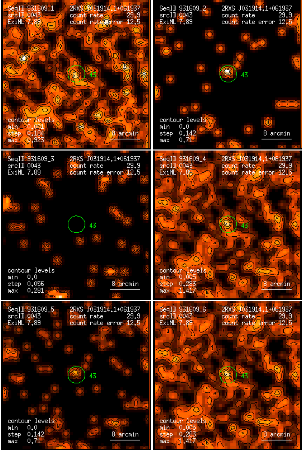
Figure 43: RASS 931609: detection 0043: band rate images, Gaussian filter: (1) PSPC channels 11 – 41, (2) 52 – 90, (3) 91 – 201, (4) 11 – 235, (5) 52 – 201, (6) 11 – 201. Broad band rates in counts/ks. Band rate contour levels in counts/ks/arcmin 2 .
