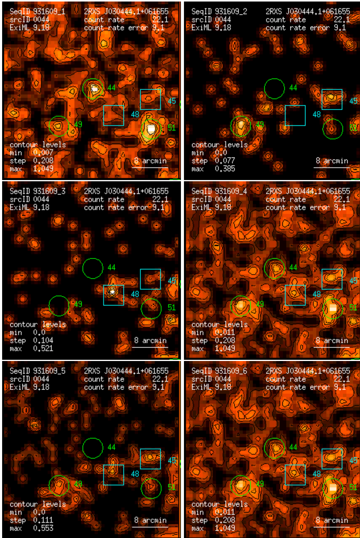
Figure 44: RASS 931609: detection 0044: band rate images, Gaussian filter: (1) PSPC channels 11 – 41, (2) 52 – 90, (3) 91 – 201, (4) 11 – 235, (5) 52 – 201, (6) 11 – 201. Broad band rates in counts/ks. Band rate contour levels in counts/ks/arcmin 2 .
