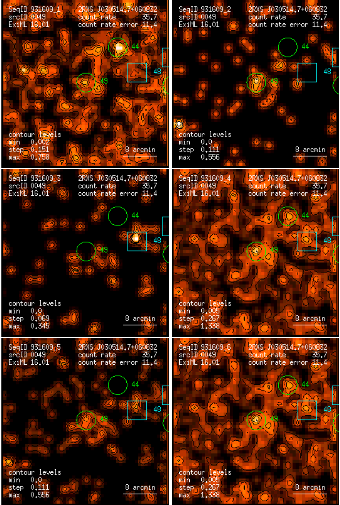
Figure 49: RASS 931609: detection 0049: band rate images, Gaussian filter: (1) PSPC channels 11 – 41, (2) 52 – 90, (3) 91 – 201, (4) 11 – 235, (5) 52 – 201, (6) 11 – 201. Broad band rates in counts/ks. Band rate contour levels in counts/ks/arcmin 2 .
