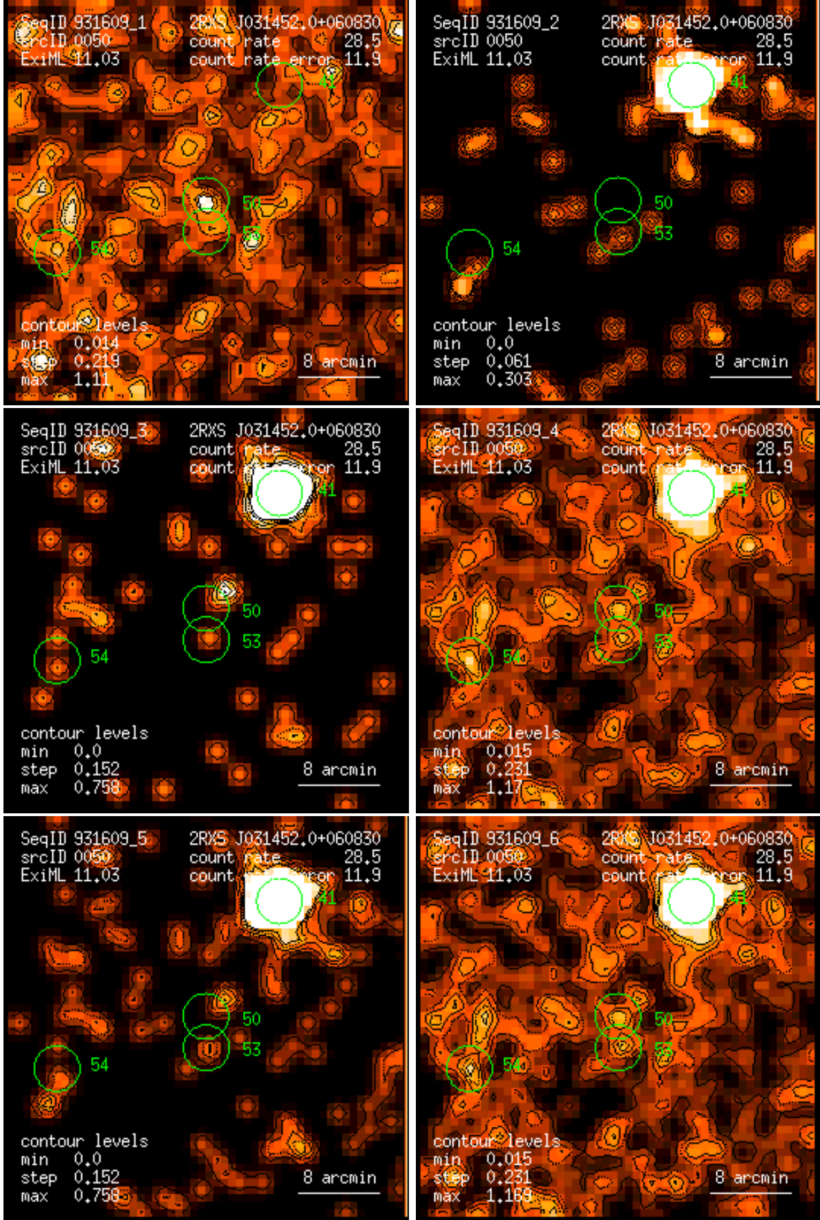
Figure 50: RASS 931609: detection 0050: band rate images, Gaussian filter: (1) PSPC channels 11 – 41, (2) 52 – 90, (3) 91 – 201, (4) 11 – 235, (5) 52 – 201, (6) 11 – 201. Broad band rates in counts/ks. Band rate contour levels in counts/ks/arcmin 2 .
