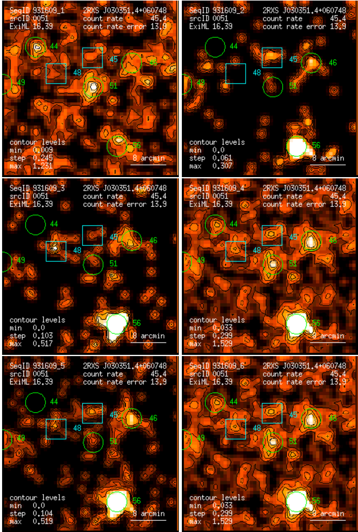
Figure 51: RASS 931609: detection 0051: band rate images, Gaussian filter: (1) PSPC channels 11 – 41, (2) 52 – 90, (3) 91 – 201, (4) 11 – 235, (5) 52 – 201, (6) 11 – 201. Broad band rates in counts/ks. Band rate contour levels in counts/ks/arcmin 2 .
