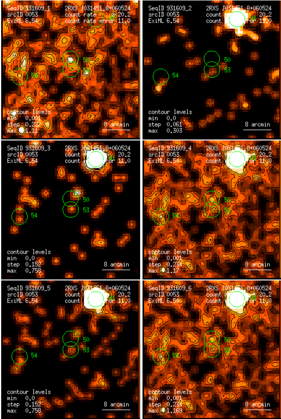
Figure 53: RASS 931609: detection 0053: band rate images, Gaussian filter: (1) PSPC channels 11 – 41, (2) 52 – 90, (3) 91 – 201, (4) 11 – 235, (5) 52 – 201, (6) 11 – 201. Broad band rates in counts/ks. Band rate contour levels in counts/ks/arcmin 2 .
