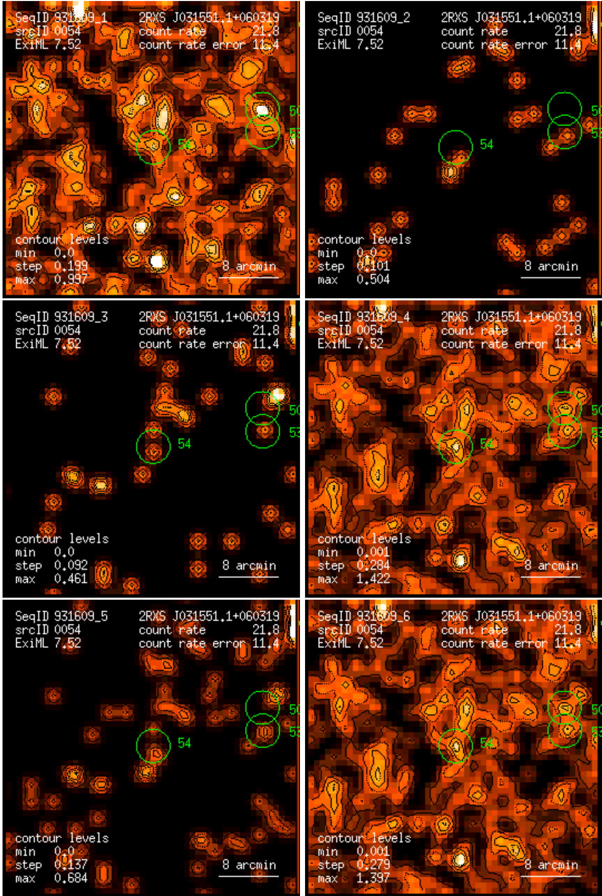
Figure 54: RASS 931609: detection 0054: band rate images, Gaussian filter: (1) PSPC channels 11 – 41, (2) 52 – 90, (3) 91 – 201, (4) 11 – 235, (5) 52 – 201, (6) 11 – 201. Broad band rates in counts/ks. Band rate contour levels in counts/ks/arcmin 2 .
