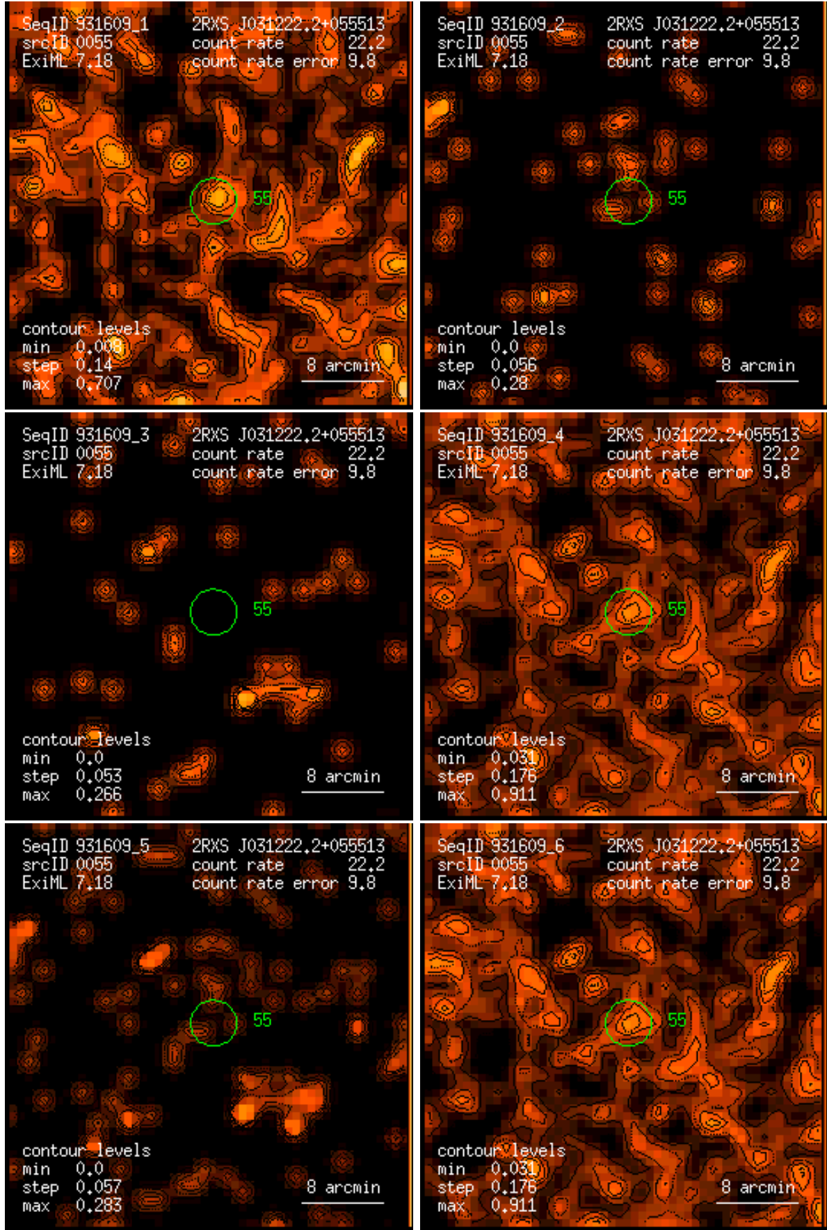
Figure 55: RASS 931609: detection 0055: band rate images, Gaussian filter: (1) PSPC channels 11 – 41, (2) 52 – 90, (3) 91 – 201, (4) 11 – 235, (5) 52 – 201, (6) 11 – 201. Broad band rates in counts/ks. Band rate contour levels in counts/ks/arcmin 2 .
