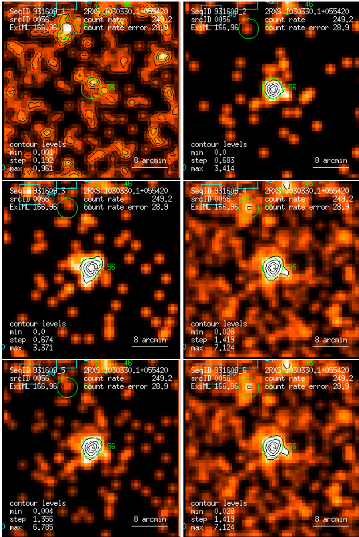
Figure 56: RASS 931609: detection 0056: band rate images, Gaussian filter: (1) PSPC channels 11 – 41, (2) 52 – 90, (3) 91 – 201, (4) 11 – 235, (5) 52 – 201, (6) 11 – 201. Broad band rates in counts/ks. Band rate contour levels in counts/ks/arcmin 2 .
