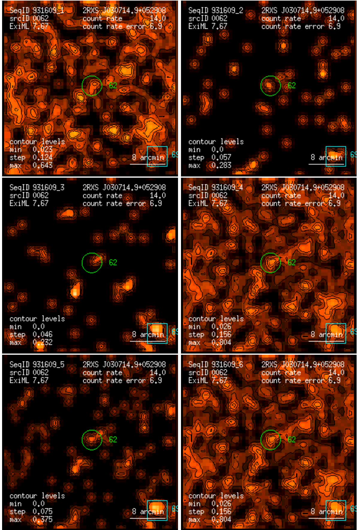
Figure 62: RASS 931609: detection 0062: band rate images, Gaussian filter: (1) PSPC channels 11 – 41, (2) 52 – 90, (3) 91 – 201, (4) 11 – 235, (5) 52 – 201, (6) 11 – 201. Broad band rates in counts/ks. Band rate contour levels in counts/ks/arcmin 2 .
