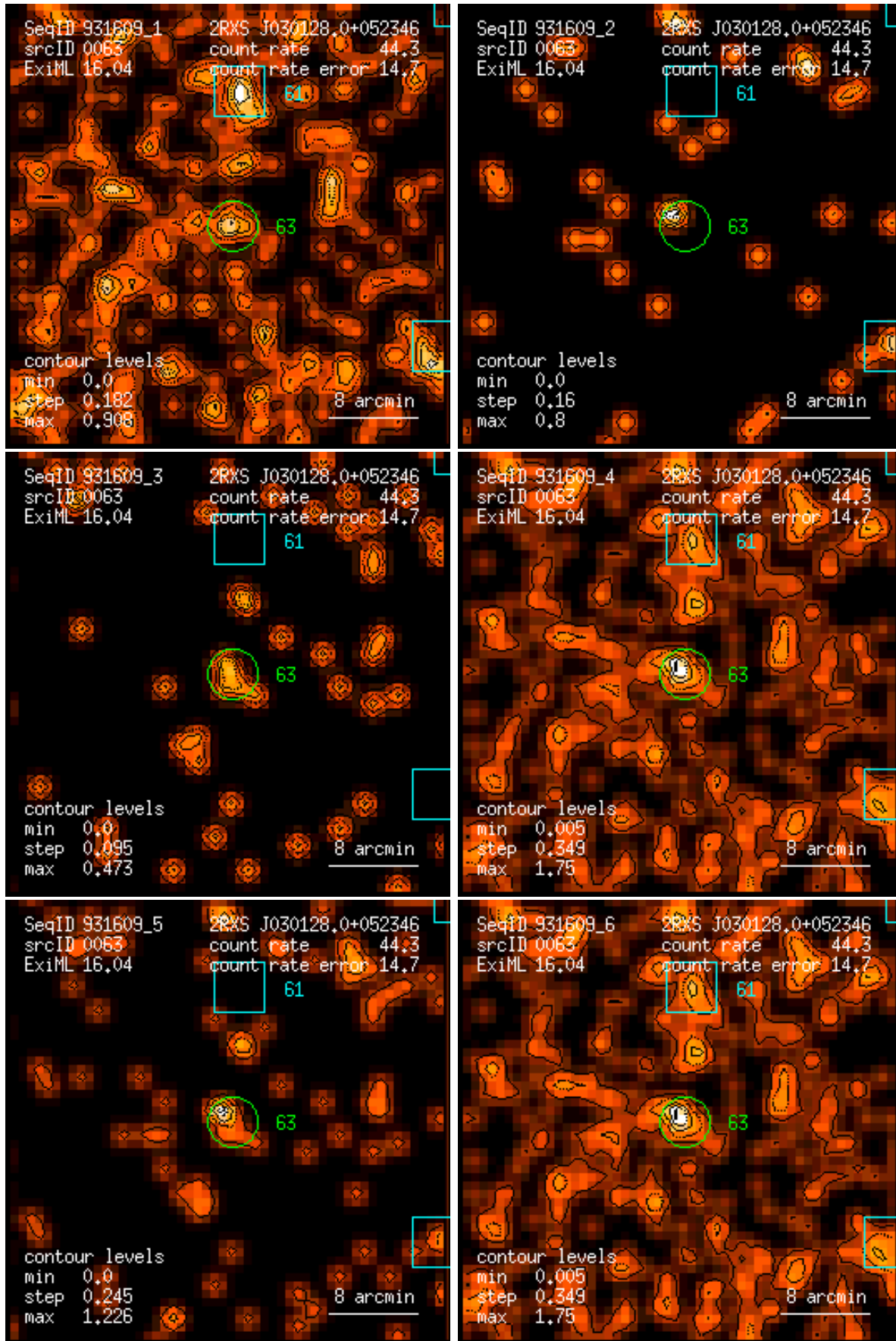
Figure 63: RASS 931609: detection 0063: band rate images, Gaussian filter: (1) PSPC channels 11 – 41, (2) 52 – 90, (3) 91 – 201, (4) 11 – 235, (5) 52 – 201, (6) 11 – 201. Broad band rates in counts/ks. Band rate contour levels in counts/ks/arcmin 2 .
