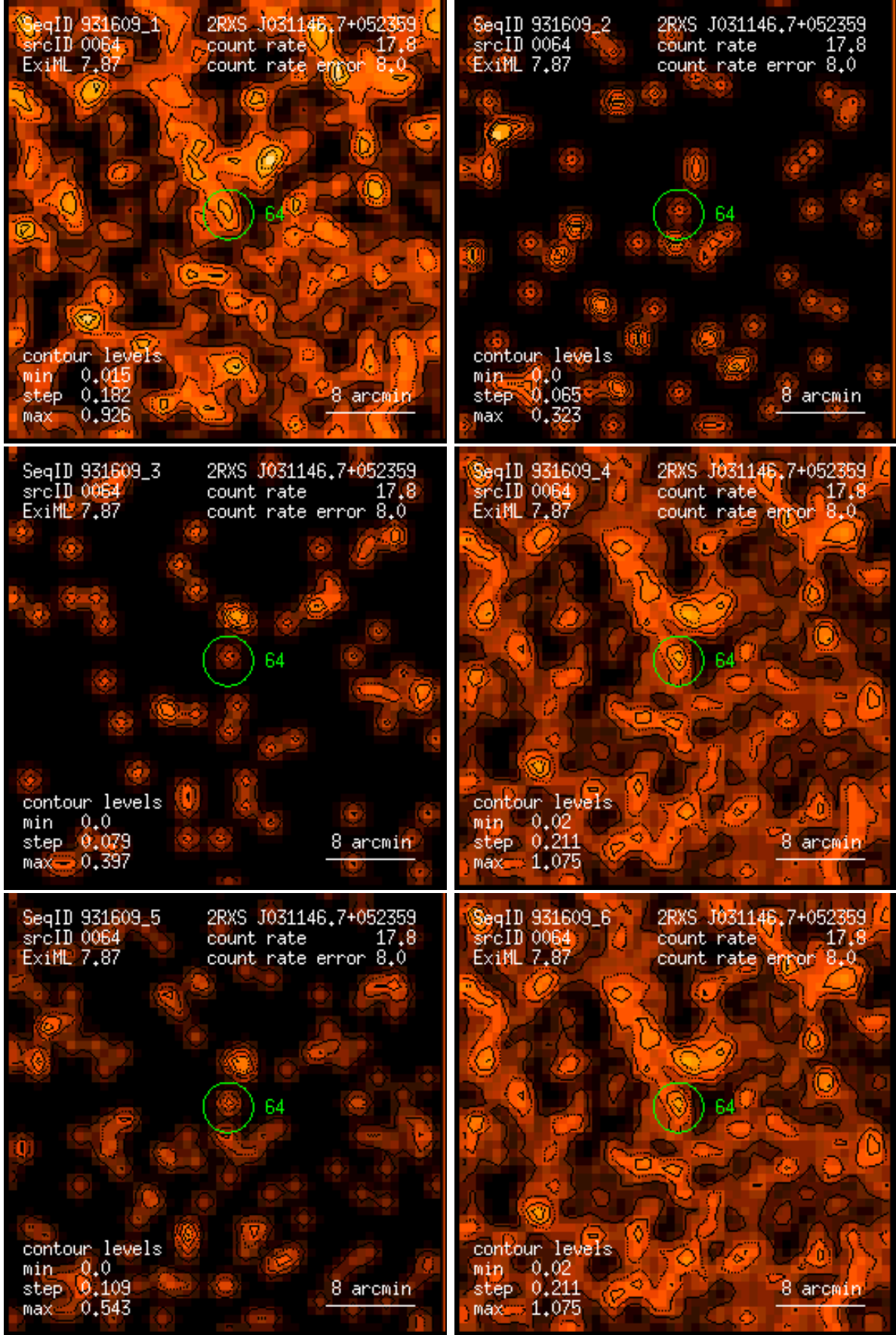
Figure 64: RASS 931609: detection 0064: band rate images, Gaussian filter: (1) PSPC channels 11 – 41, (2) 52 – 90, (3) 91 – 201, (4) 11 – 235, (5) 52 – 201, (6) 11 – 201. Broad band rates in counts/ks. Band rate contour levels in counts/ks/arcmin 2 .
