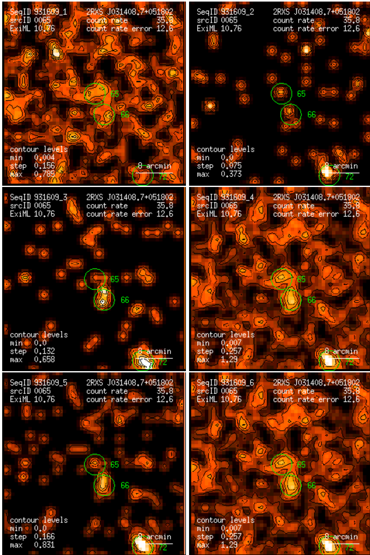
Figure 65: RASS 931609: detection 0065: band rate images, Gaussian filter: (1) PSPC channels 11 – 41, (2) 52 – 90, (3) 91 – 201, (4) 11 – 235, (5) 52 – 201, (6) 11 – 201. Broad band rates in counts/ks. Band rate contour levels in counts/ks/arcmin 2 .
