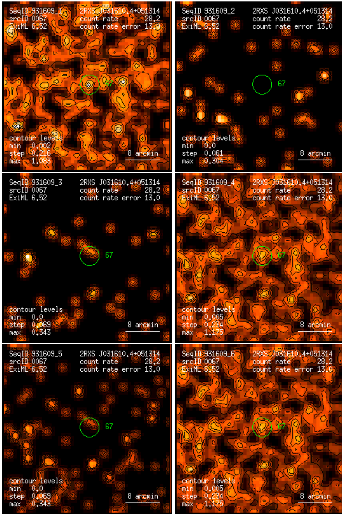
Figure 67: RASS 931609: detection 0067: band rate images, Gaussian filter: (1) PSPC channels 11 – 41, (2) 52 – 90, (3) 91 – 201, (4) 11 – 235, (5) 52 – 201, (6) 11 – 201. Broad band rates in counts/ks. Band rate contour levels in counts/ks/arcmin 2 .
