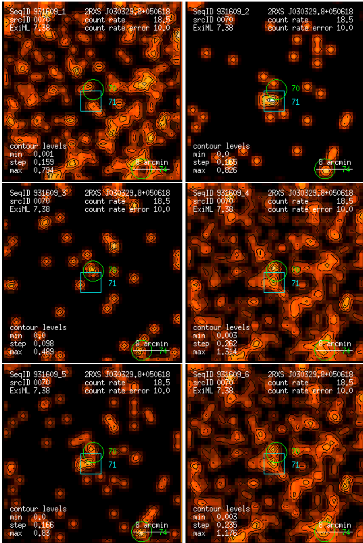
Figure 70: RASS 931609: detection 0070: band rate images, Gaussian filter: (1) PSPC channels 11 – 41, (2) 52 – 90, (3) 91 – 201, (4) 11 – 235, (5) 52 – 201, (6) 11 – 201. Broad band rates in counts/ks. Band rate contour levels in counts/ks/arcmin 2 .
