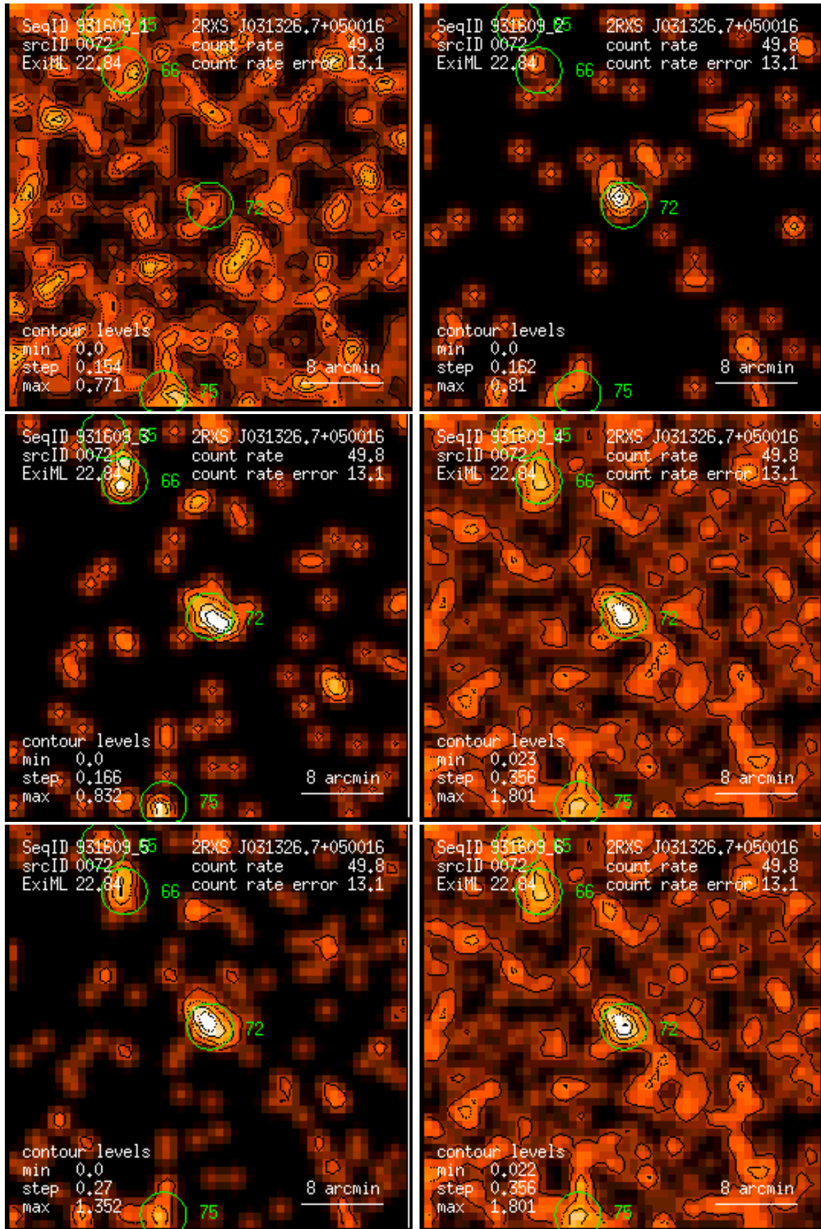
Figure 72: RASS 931609: detection 0072: band rate images, Gaussian filter: (1) PSPC channels 11 – 41, (2) 52 – 90, (3) 91 – 201, (4) 11 – 235, (5) 52 – 201, (6) 11 – 201. Broad band rates in counts/ks. Band rate contour levels in counts/ks/arcmin 2 .
