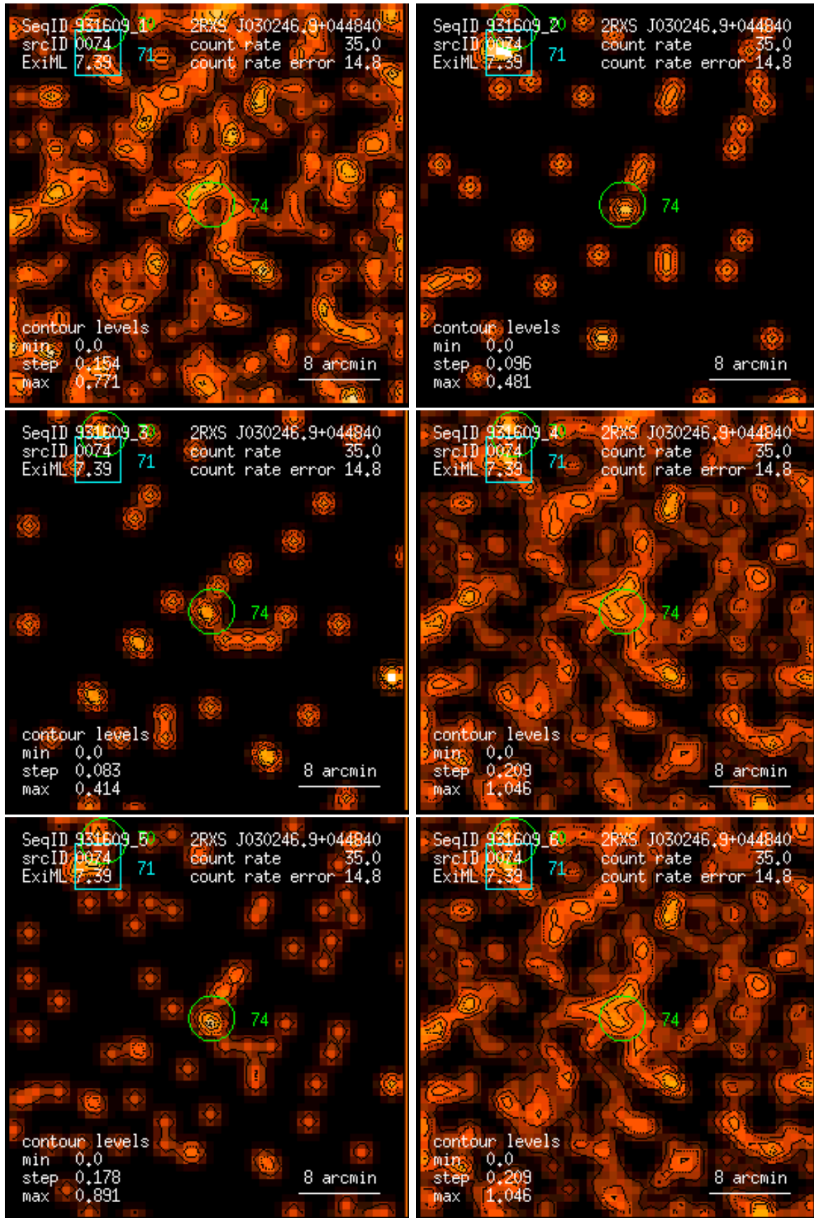
Figure 74: RASS 931609: detection 0074: band rate images, Gaussian filter: (1) PSPC channels 11 – 41, (2) 52 – 90, (3) 91 – 201, (4) 11 – 235, (5) 52 – 201, (6) 11 – 201. Broad band rates in counts/ks. Band rate contour levels in counts/ks/arcmin 2 .
