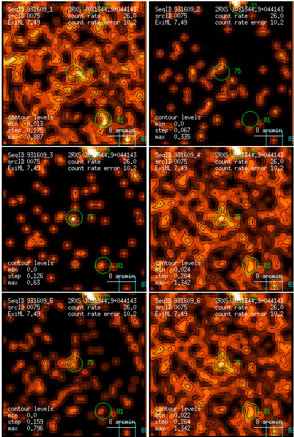
Figure 75: RASS 931609: detection 0075: band rate images, Gaussian filter: (1) PSPC channels 11 – 41, (2) 52 – 90, (3) 91 – 201, (4) 11 – 235, (5) 52 – 201, (6) 11 – 201. Broad band rates in counts/ks. Band rate contour levels in counts/ks/arcmin 2 .
