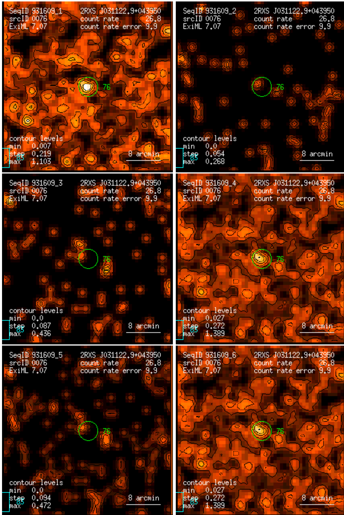
Figure 76: RASS 931609: detection 0076: band rate images, Gaussian filter: (1) PSPC channels 11 – 41, (2) 52 – 90, (3) 91 – 201, (4) 11 – 235, (5) 52 – 201, (6) 11 – 201. Broad band rates in counts/ks. Band rate contour levels in counts/ks/arcmin 2 .
