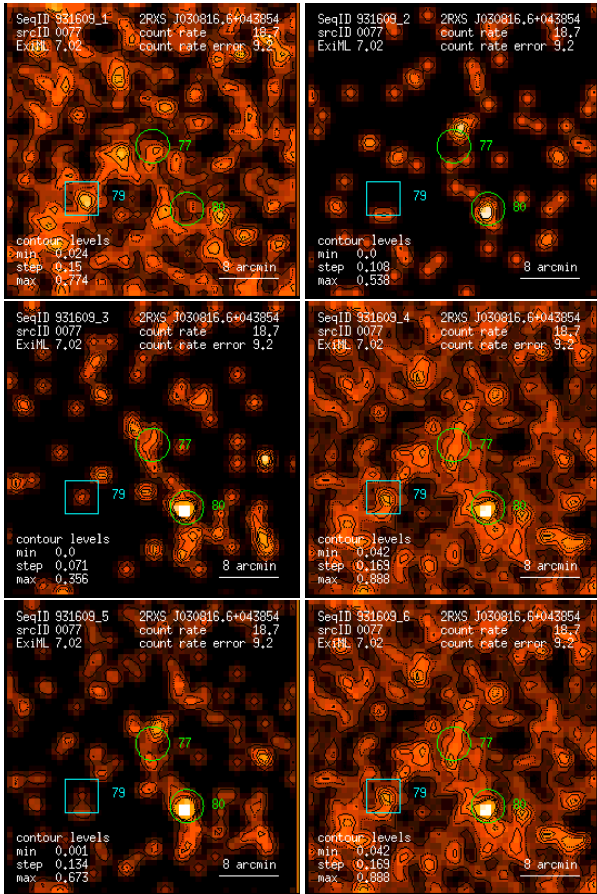
Figure 77: RASS 931609: detection 0077: band rate images, Gaussian filter: (1) PSPC channels 11 – 41, (2) 52 – 90, (3) 91 – 201, (4) 11 – 235, (5) 52 – 201, (6) 11 – 201. Broad band rates in counts/ks. Band rate contour levels in counts/ks/arcmin 2 .
