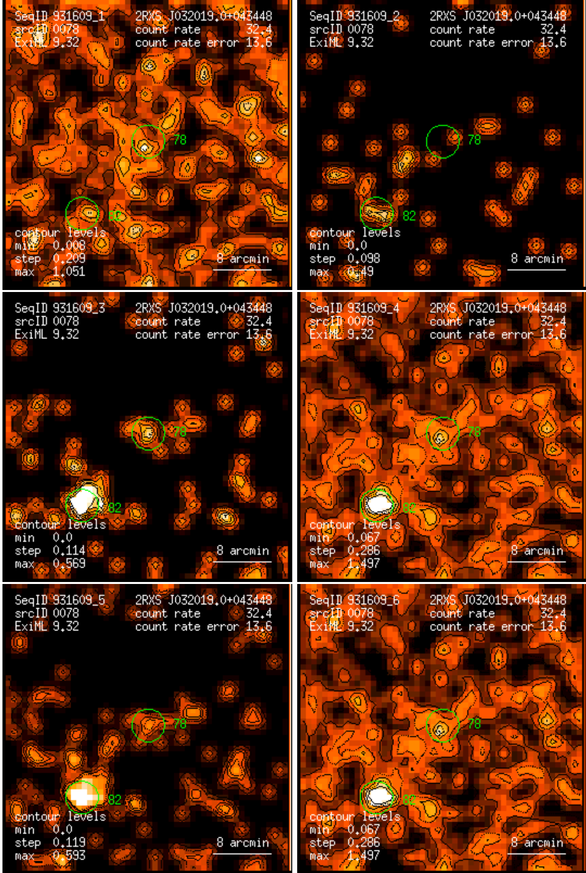
Figure 78: RASS 931609: detection 0078: band rate images, Gaussian filter: (1) PSPC channels 11 – 41, (2) 52 – 90, (3) 91 – 201, (4) 11 – 235, (5) 52 – 201, (6) 11 – 201. Broad band rates in counts/ks. Band rate contour levels in counts/ks/arcmin 2 .
