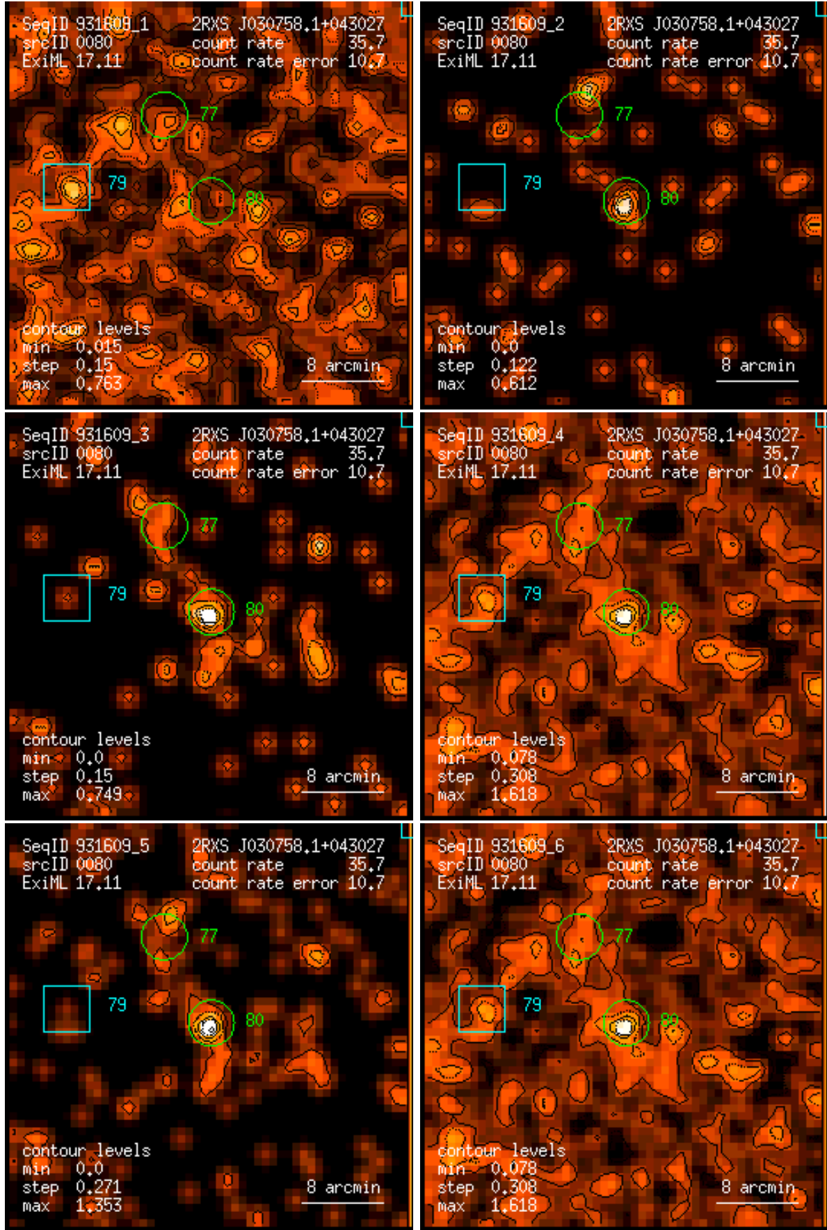
Figure 80: RASS 931609: detection 0080: band rate images, Gaussian filter: (1) PSPC channels 11 – 41, (2) 52 – 90, (3) 91 – 201, (4) 11 – 235, (5) 52 – 201, (6) 11 – 201. Broad band rates in counts/ks. Band rate contour levels in counts/ks/arcmin 2 .
