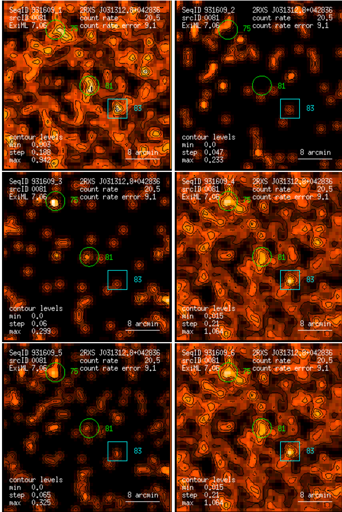
Figure 81: RASS 931609: detection 0081: band rate images, Gaussian filter: (1) PSPC channels 11 – 41, (2) 52 – 90, (3) 91 – 201, (4) 11 – 235, (5) 52 – 201, (6) 11 – 201. Broad band rates in counts/ks. Band rate contour levels in counts/ks/arcmin 2 .
