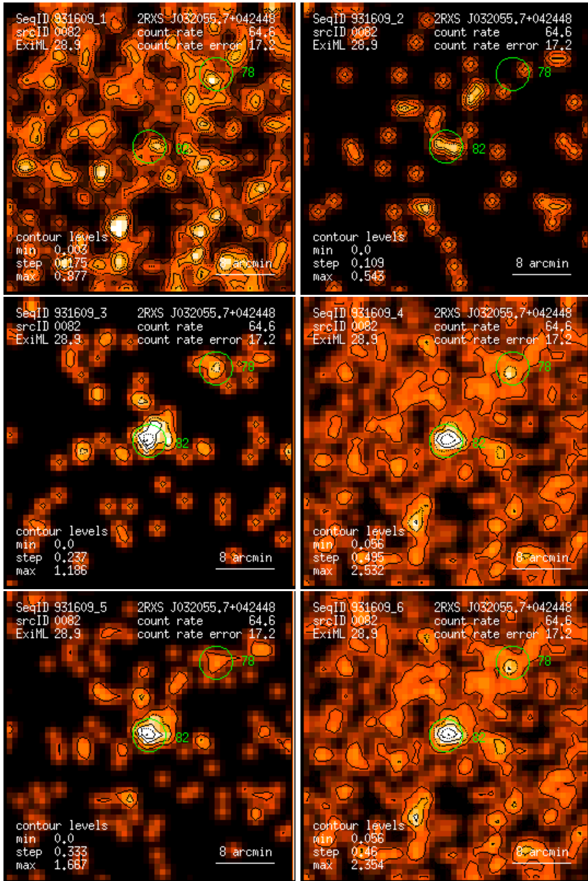
Figure 82: RASS 931609: detection 0082: band rate images, Gaussian filter: (1) PSPC channels 11 – 41, (2) 52 – 90, (3) 91 – 201, (4) 11 – 235, (5) 52 – 201, (6) 11 – 201. Broad band rates in counts/ks. Band rate contour levels in counts/ks/arcmin 2 .
