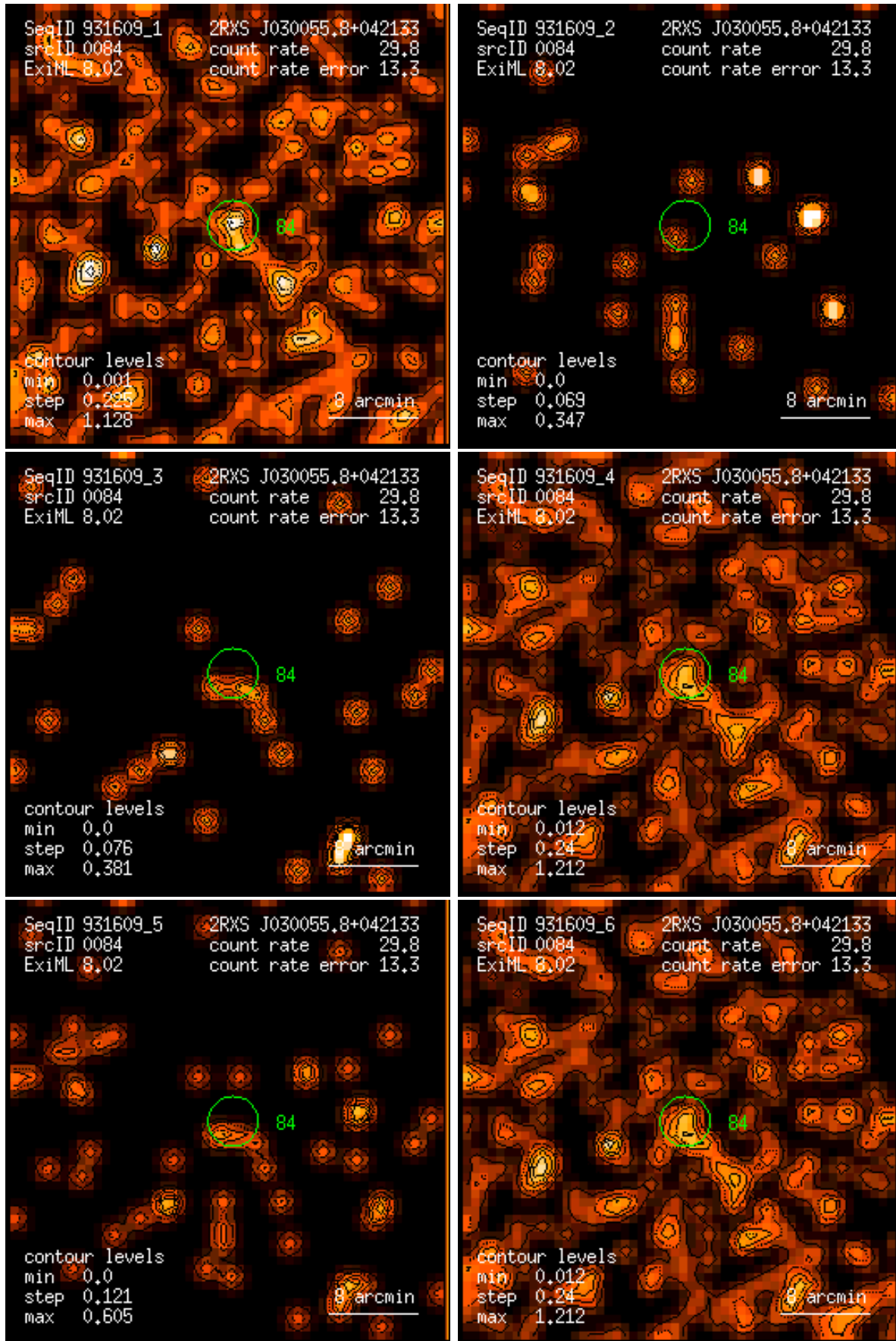
Figure 84: RASS 931609: detection 0084: band rate images, Gaussian filter: (1) PSPC channels 11 – 41, (2) 52 – 90, (3) 91 – 201, (4) 11 – 235, (5) 52 – 201, (6) 11 – 201. Broad band rates in counts/ks. Band rate contour levels in counts/ks/arcmin 2 .
