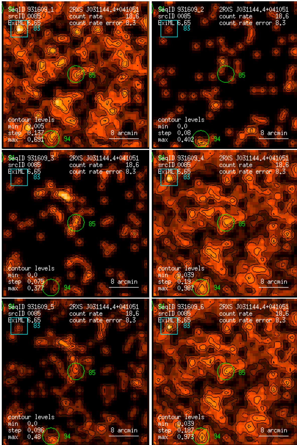
Figure 85: RASS 931609: detection 0085: band rate images, Gaussian filter: (1) PSPC channels 11 – 41, (2) 52 – 90, (3) 91 – 201, (4) 11 – 235, (5) 52 – 201, (6) 11 – 201. Broad band rates in counts/ks. Band rate contour levels in counts/ks/arcmin 2 .
