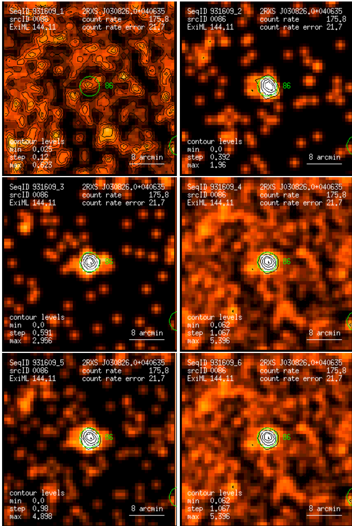
Figure 86: RASS 931609: detection 0086: band rate images, Gaussian filter: (1) PSPC channels 11 – 41, (2) 52 – 90, (3) 91 – 201, (4) 11 – 235, (5) 52 – 201, (6) 11 – 201. Broad band rates in counts/ks. Band rate contour levels in counts/ks/arcmin 2 .
