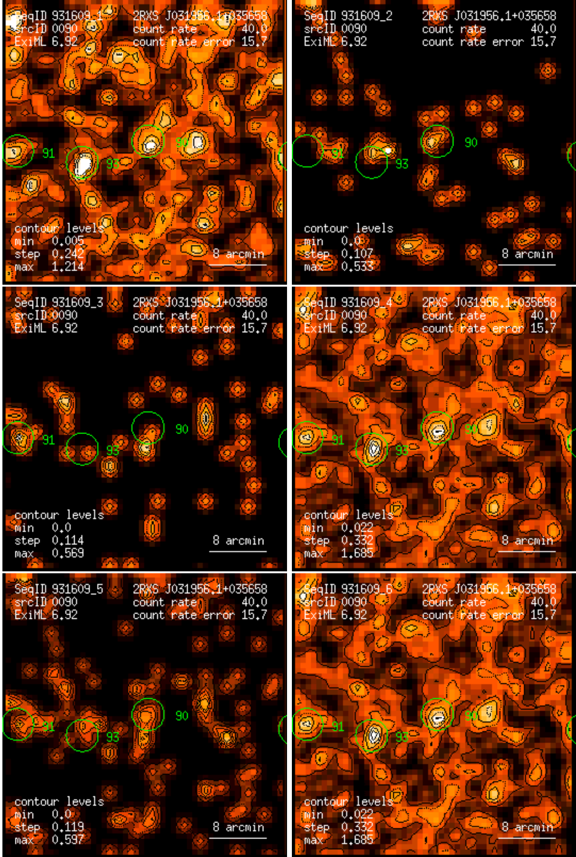
Figure 90: RASS 931609: detection 0090: band rate images, Gaussian filter: (1) PSPC channels 11 – 41, (2) 52 – 90, (3) 91 – 201, (4) 11 – 235, (5) 52 – 201, (6) 11 – 201. Broad band rates in counts/ks. Band rate contour levels in counts/ks/arcmin 2 .
