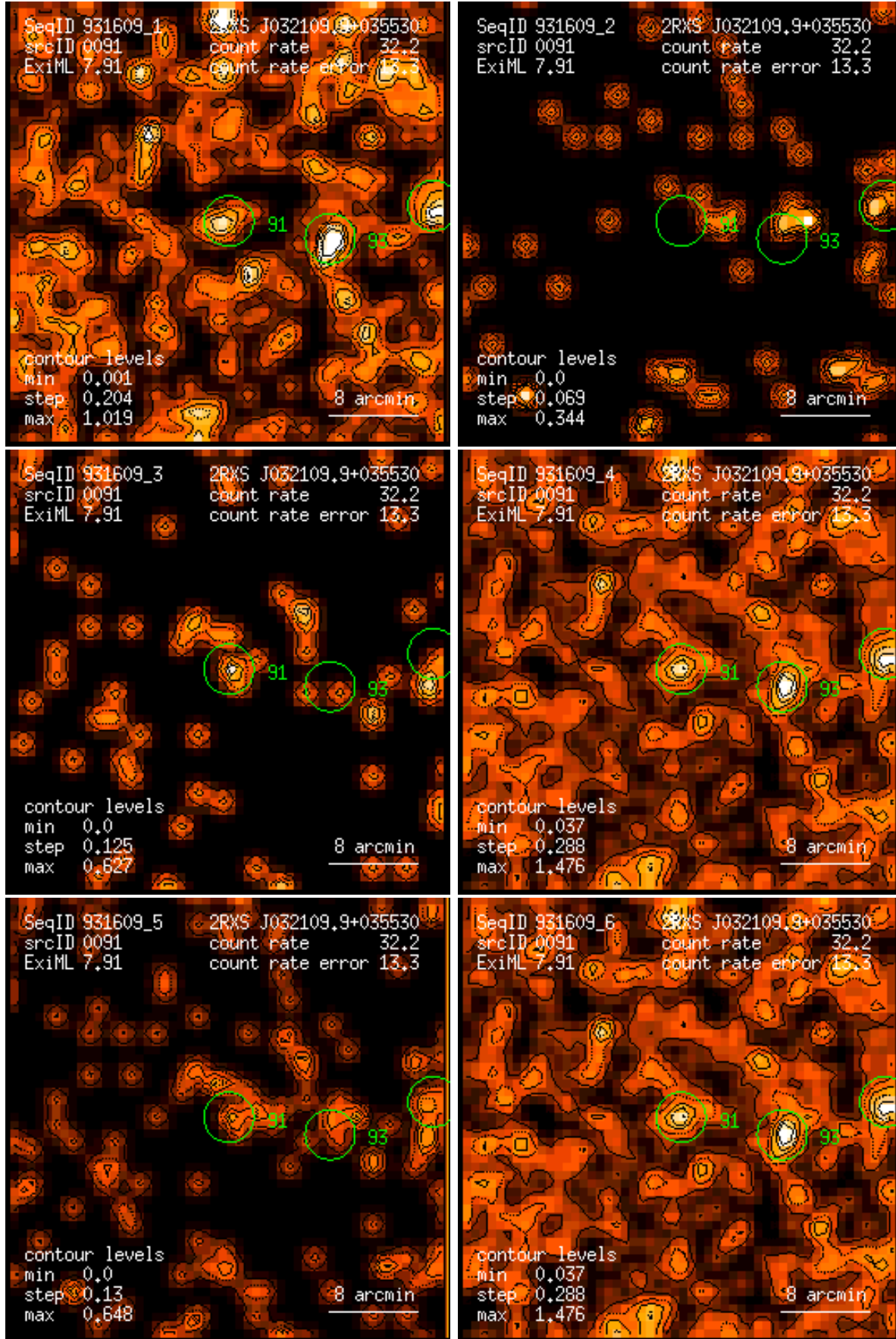
Figure 91: RASS 931609: detection 0091: band rate images, Gaussian filter: (1) PSPC channels 11 – 41, (2) 52 – 90, (3) 91 – 201, (4) 11 – 235, (5) 52 – 201, (6) 11 – 201. Broad band rates in counts/ks. Band rate contour levels in counts/ks/arcmin 2 .
