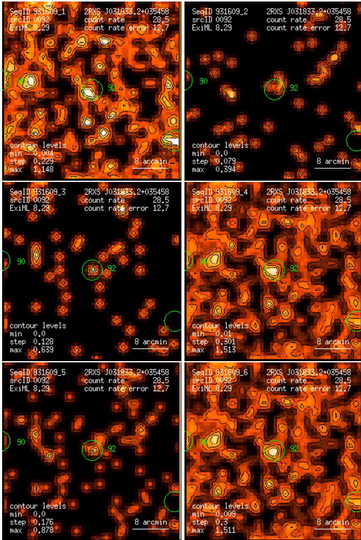
Figure 92: RASS 931609: detection 0092: band rate images, Gaussian filter: (1) PSPC channels 11 – 41, (2) 52 – 90, (3) 91 – 201, (4) 11 – 235, (5) 52 – 201, (6) 11 – 201. Broad band rates in counts/ks. Band rate contour levels in counts/ks/arcmin 2 .
