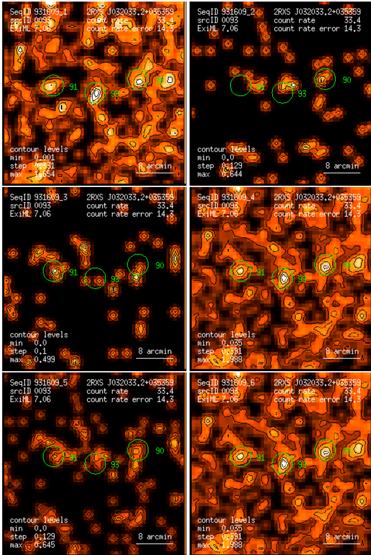
Figure 93: RASS 931609: detection 0093: band rate images, Gaussian filter: (1) PSPC channels 11 – 41, (2) 52 – 90, (3) 91 – 201, (4) 11 – 235, (5) 52 – 201, (6) 11 – 201. Broad band rates in counts/ks. Band rate contour levels in counts/ks/arcmin 2 .
