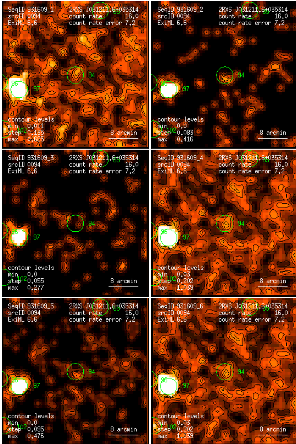
Figure 94: RASS 931609: detection 0094: band rate images, Gaussian filter: (1) PSPC channels 11 – 41, (2) 52 – 90, (3) 91 – 201, (4) 11 – 235, (5) 52 – 201, (6) 11 – 201. Broad band rates in counts/ks. Band rate contour levels in counts/ks/arcmin 2 .
