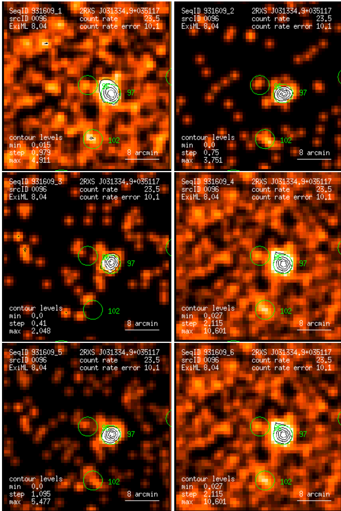
Figure 96: RASS 931609: detection 0096: band rate images, Gaussian filter: (1) PSPC channels 11 – 41, (2) 52 – 90, (3) 91 – 201, (4) 11 – 235, (5) 52 – 201, (6) 11 – 201. Broad band rates in counts/ks. Band rate contour levels in counts/ks/arcmin 2 .
