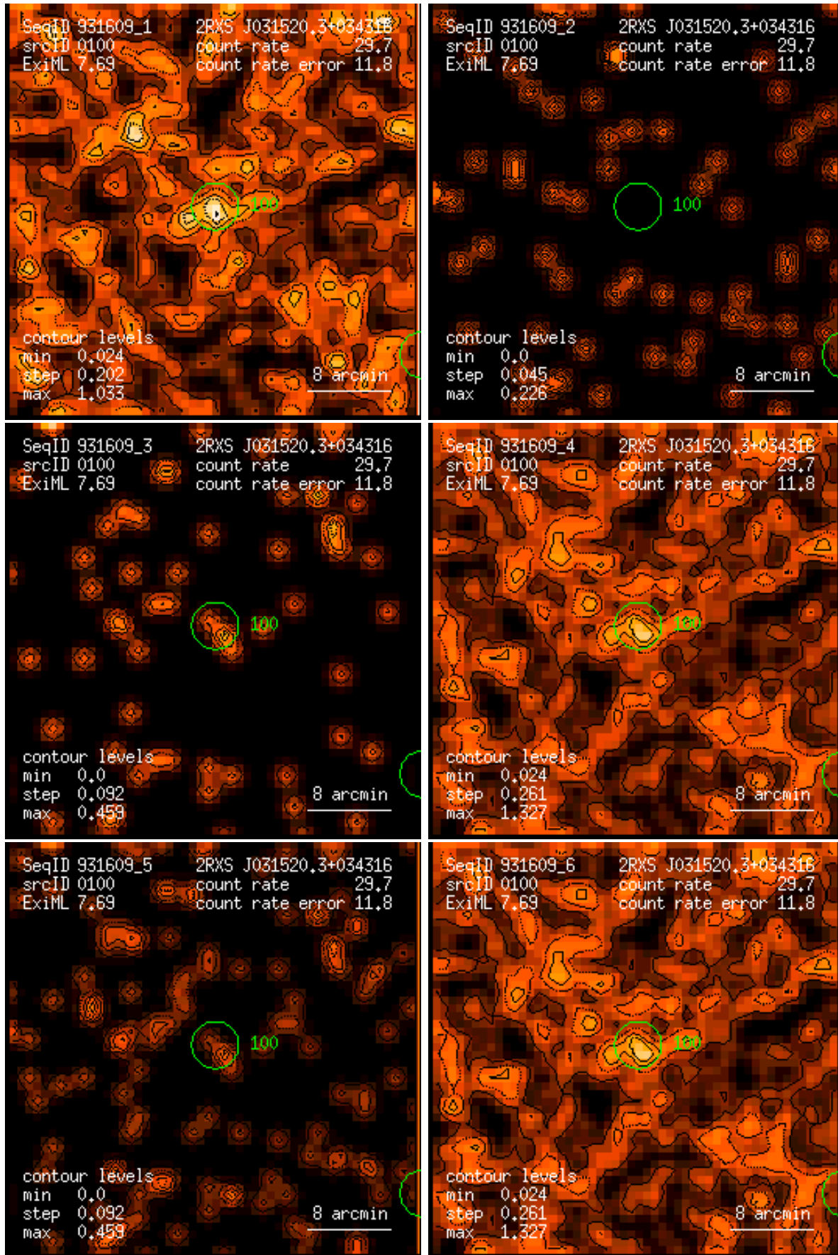
Figure 100: RASS 931609: detection 0100: band rate images, Gaussian filter: (1) PSPC channels 11 – 41, (2) 52 – 90, (3) 91 – 201, (4) 11 – 235, (5) 52 – 201, (6) 11 – 201. Broad band rates in counts/ks. Band rate contour levels in counts/ks/arcmin 2 .
