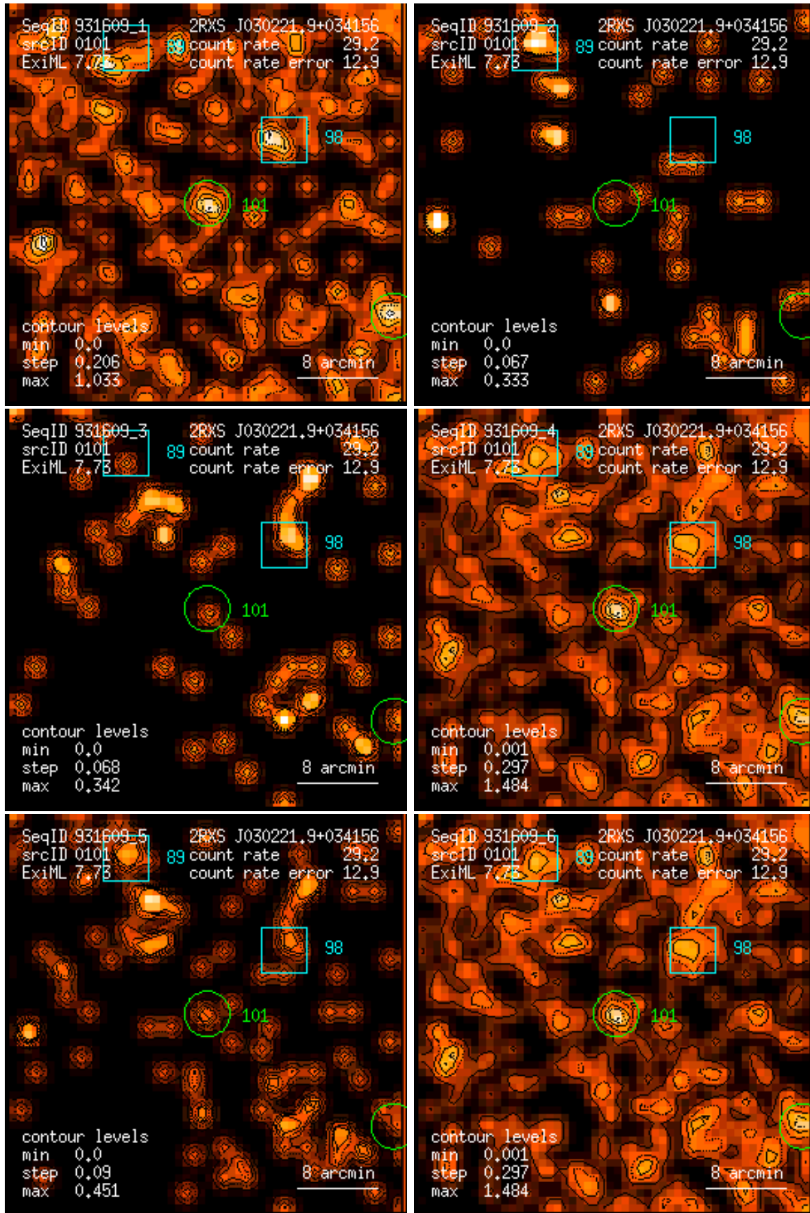
Figure 101: RASS 931609: detection 0101: band rate images, Gaussian filter: (1) PSPC channels 11 – 41, (2) 52 – 90, (3) 91 – 201, (4) 11 – 235, (5) 52 – 201, (6) 11 – 201. Broad band rates in counts/ks. Band rate contour levels in counts/ks/arcmin 2 .
