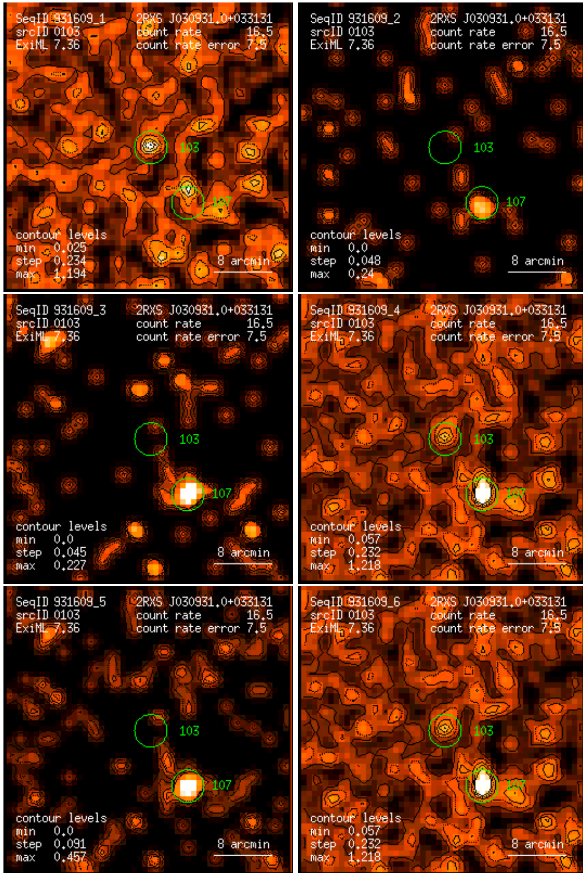
Figure 103: RASS 931609: detection 0103: band rate images, Gaussian filter: (1) PSPC channels 11 – 41, (2) 52 – 90, (3) 91 – 201, (4) 11 – 235, (5) 52 – 201, (6) 11 – 201. Broad band rates in counts/ks. Band rate contour levels in counts/ks/arcmin 2 .
