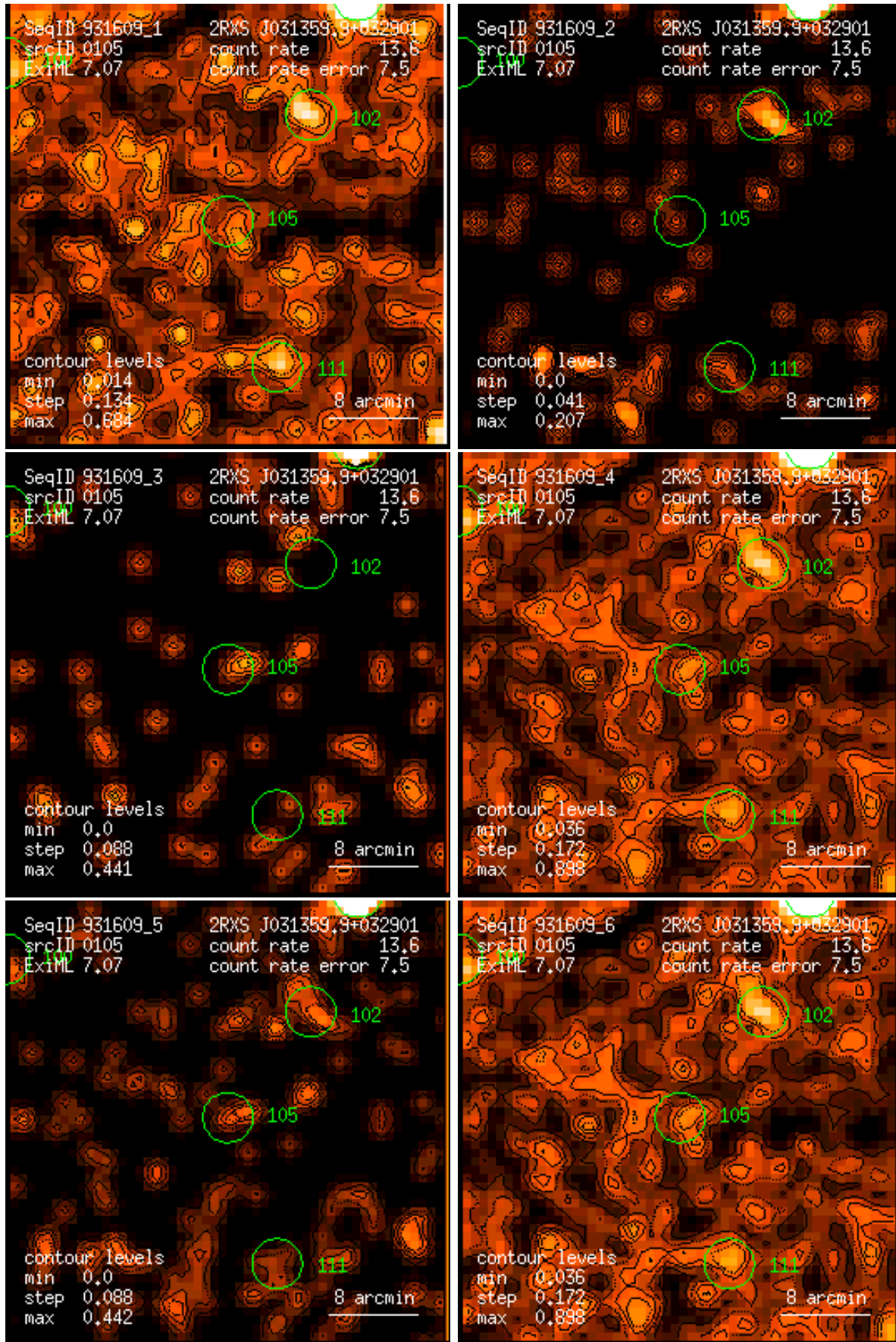
Figure 105: RASS 931609: detection 0105: band rate images, Gaussian filter: (1) PSPC channels 11 – 41, (2) 52 – 90, (3) 91 – 201, (4) 11 – 235, (5) 52 – 201, (6) 11 – 201. Broad band rates in counts/ks. Band rate contour levels in counts/ks/arcmin 2 .
