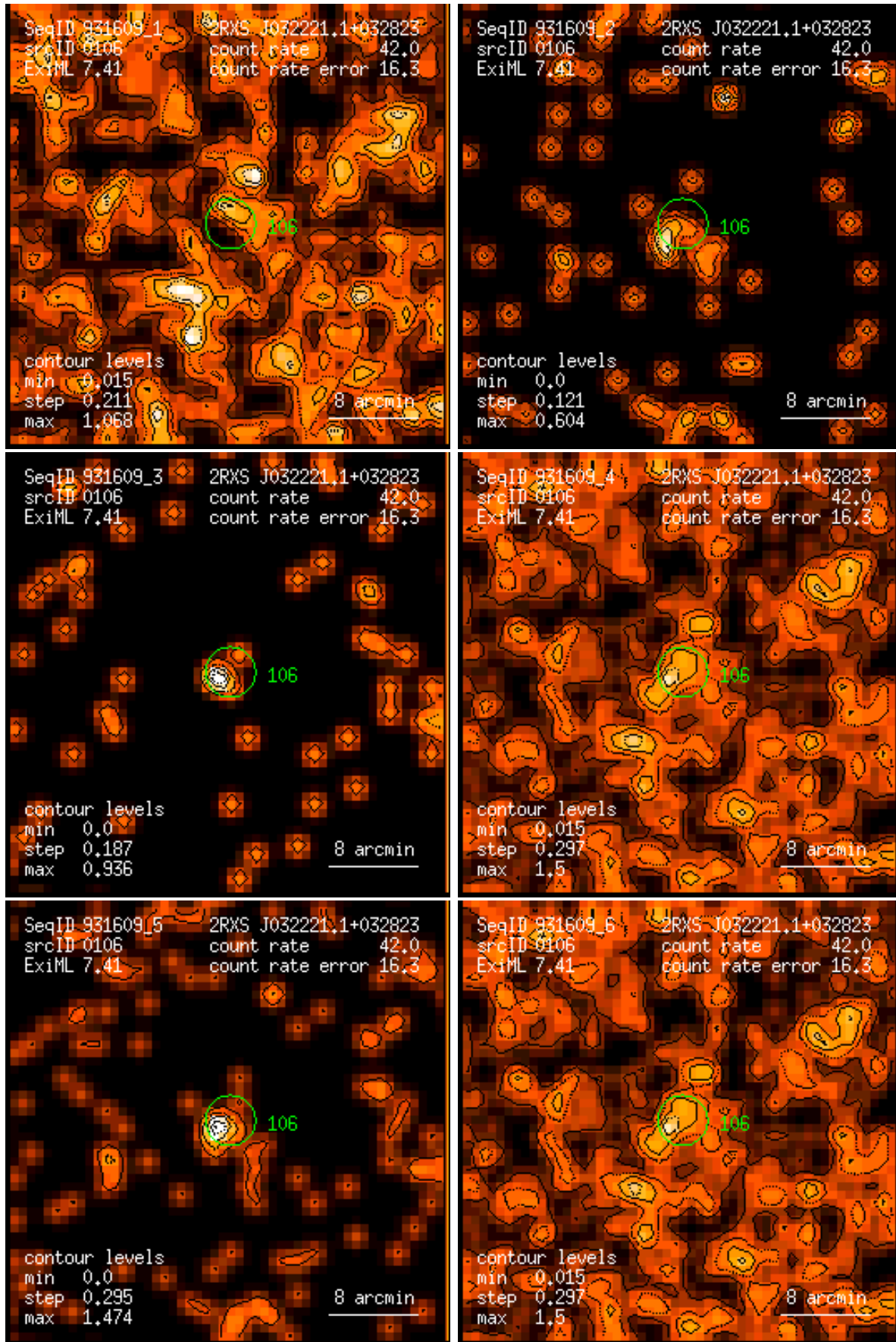
Figure 106: RASS 931609: detection 0106: band rate images, Gaussian filter: (1) PSPC channels 11 – 41, (2) 52 – 90, (3) 91 – 201, (4) 11 – 235, (5) 52 – 201, (6) 11 – 201. Broad band rates in counts/ks. Band rate contour levels in counts/ks/arcmin 2 .
