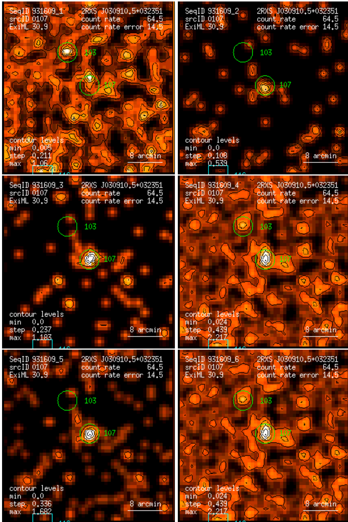
Figure 107: RASS 931609: detection 0107: band rate images, Gaussian filter: (1) PSPC channels 11 – 41, (2) 52 – 90, (3) 91 – 201, (4) 11 – 235, (5) 52 – 201, (6) 11 – 201. Broad band rates in counts/ks. Band rate contour levels in counts/ks/arcmin 2 .
