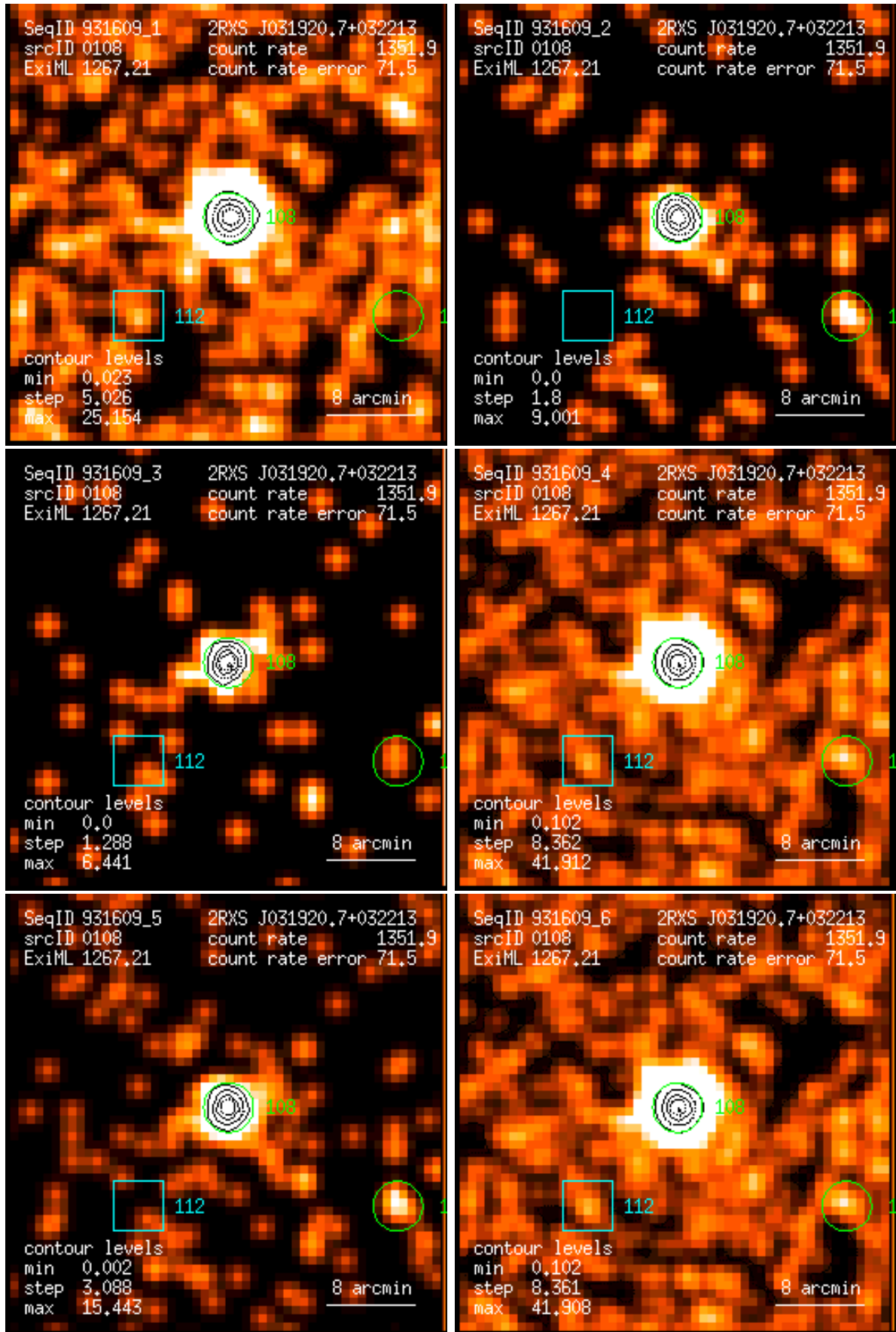
Figure 108: RASS 931609: detection 0108: band rate images, Gaussian filter: (1) PSPC channels 11 – 41, (2) 52 – 90, (3) 91 – 201, (4) 11 – 235, (5) 52 – 201, (6) 11 – 201. Broad band rates in counts/ks. Band rate contour levels in counts/ks/arcmin 2 .
