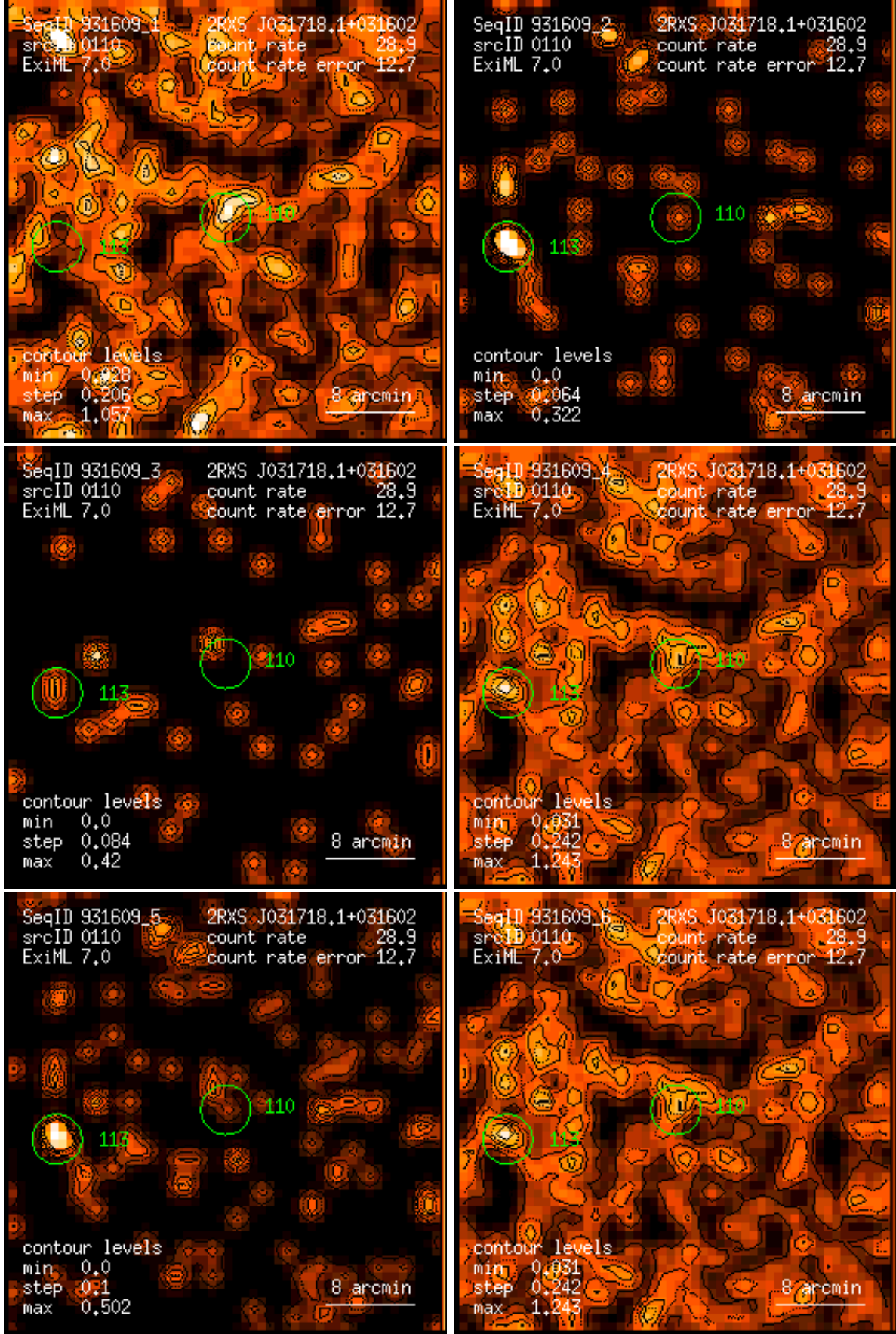
Figure 110: RASS 931609: detection 0110: band rate images, Gaussian filter: (1) PSPC channels 11 – 41, (2) 52 – 90, (3) 91 – 201, (4) 11 – 235, (5) 52 – 201, (6) 11 – 201. Broad band rates in counts/ks. Band rate contour levels in counts/ks/arcmin 2 .
