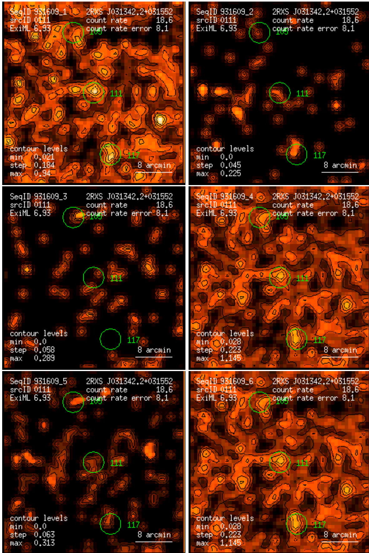
Figure 111: RASS 931609: detection 0111: band rate images, Gaussian filter: (1) PSPC channels 11 – 41, (2) 52 – 90, (3) 91 – 201, (4) 11 – 235, (5) 52 – 201, (6) 11 – 201. Broad band rates in counts/ks. Band rate contour levels in counts/ks/arcmin 2 .
