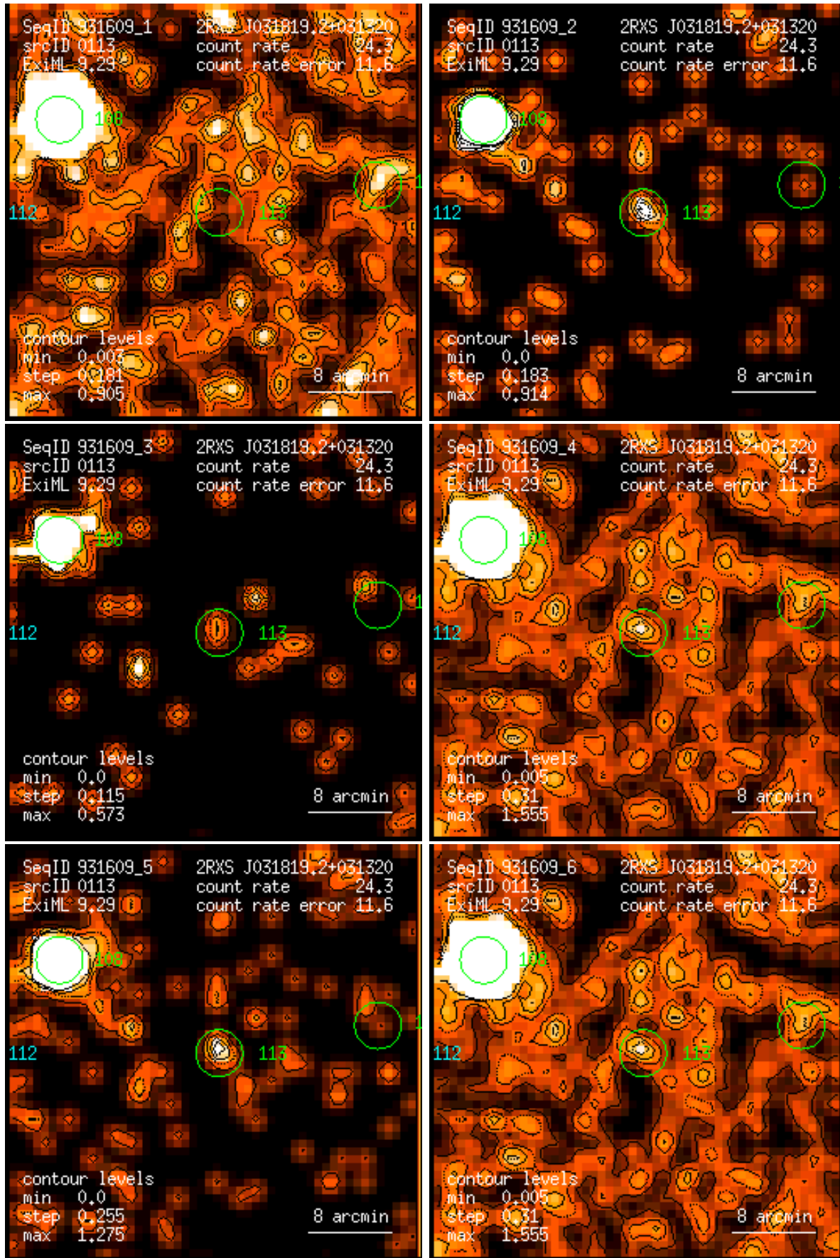
Figure 113: RASS 931609: detection 0113: band rate images, Gaussian filter: (1) PSPC channels 11 – 41, (2) 52 – 90, (3) 91 – 201, (4) 11 – 235, (5) 52 – 201, (6) 11 – 201. Broad band rates in counts/ks. Band rate contour levels in counts/ks/arcmin 2 .
