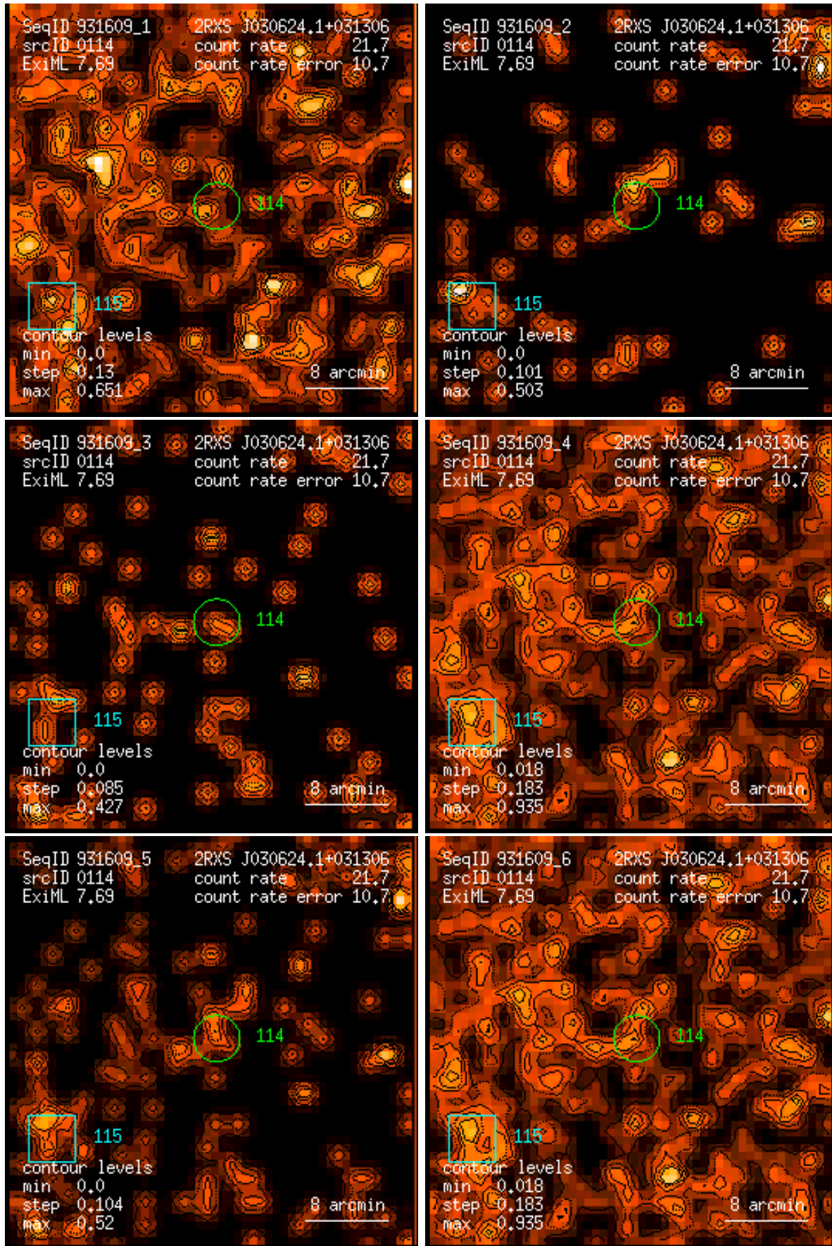
Figure 114: RASS 931609: detection 0114: band rate images, Gaussian filter: (1) PSPC channels 11 – 41, (2) 52 – 90, (3) 91 – 201, (4) 11 – 235, (5) 52 – 201, (6) 11 – 201. Broad band rates in counts/ks. Band rate contour levels in counts/ks/arcmin 2 .
